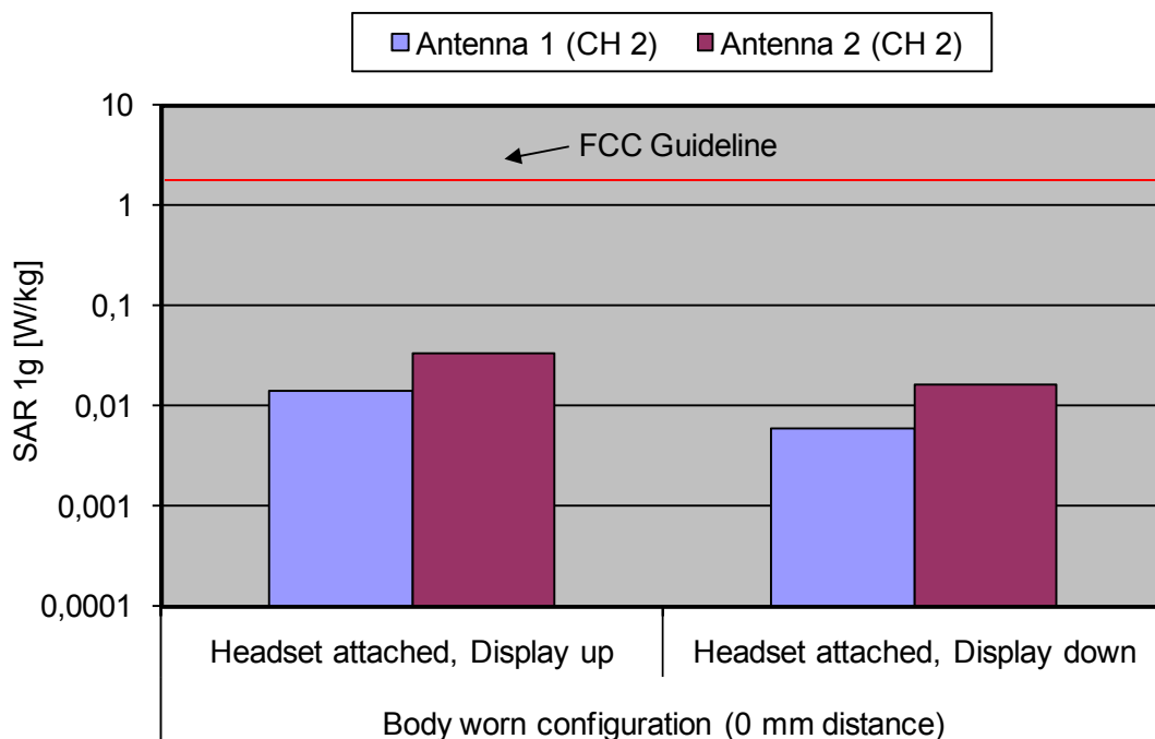
Fig. 9: The measured SAR values in body worn configuration for the RTX 8630 for the US DECT standard in comparison to the FCC exposure limit.
