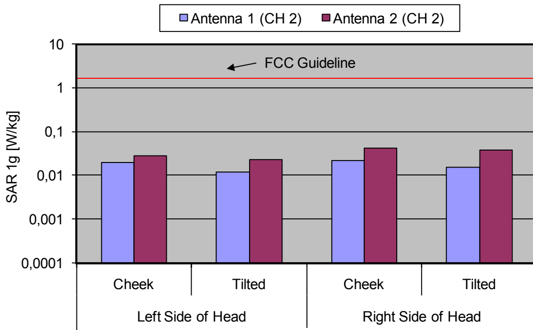
Fig. 8: The measured head phantom SAR values for the RTX 8630 for the US DECT standard in comparison to the FCC exposure limit.
