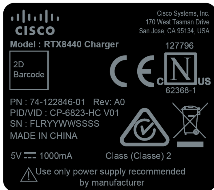
EUT – Charger Label 1 View
