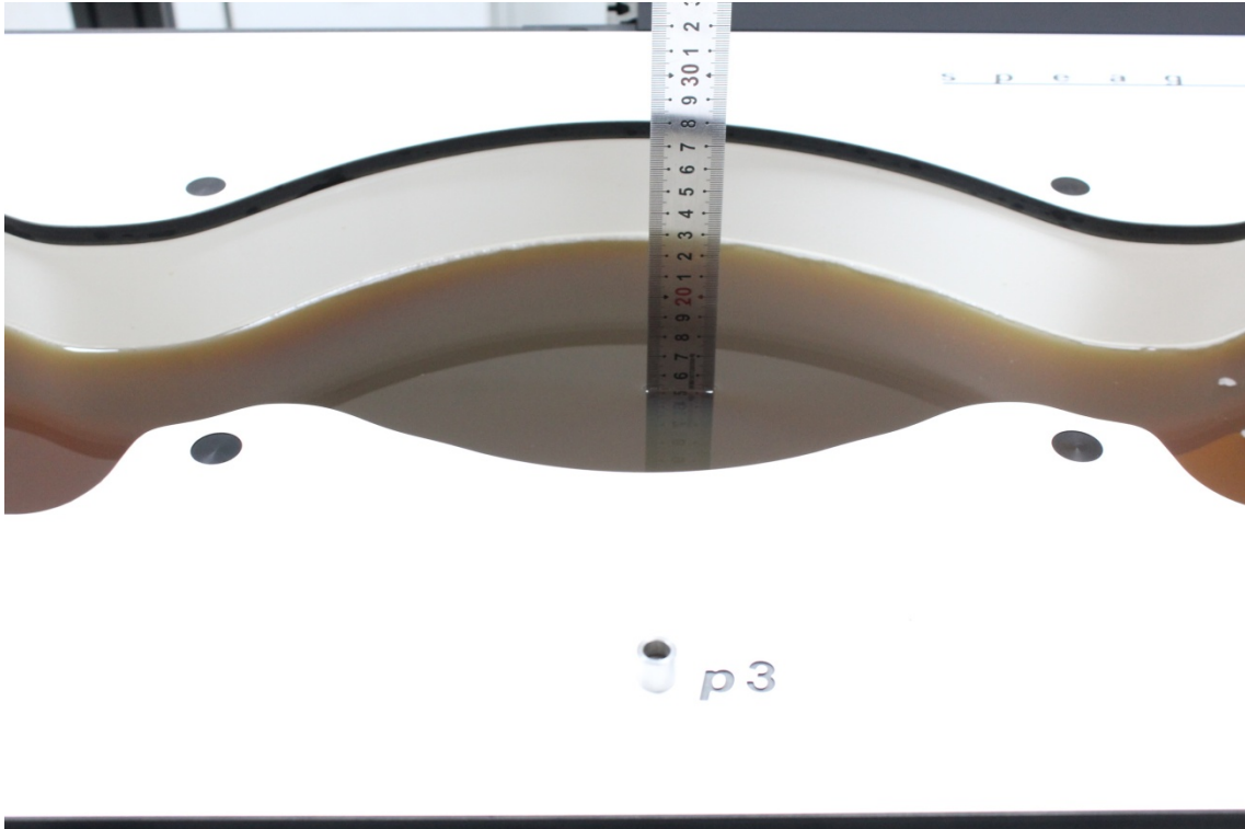
Body Back Setup Photo (0mm) (Model: 8254 DECT Handset)
