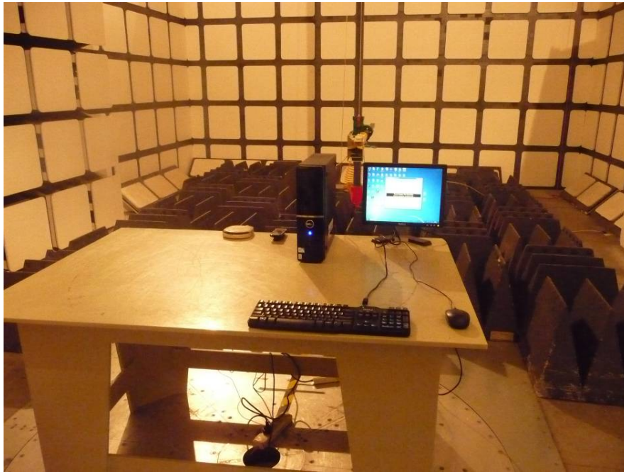
Above 1 GHz: Radiated Emissions – Front View (Downloading mode)
