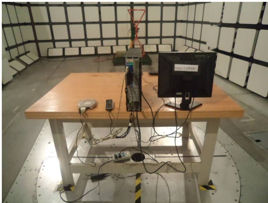
Below 1 GHz: Radiated Emissions – Rear View (Downloading mode)
