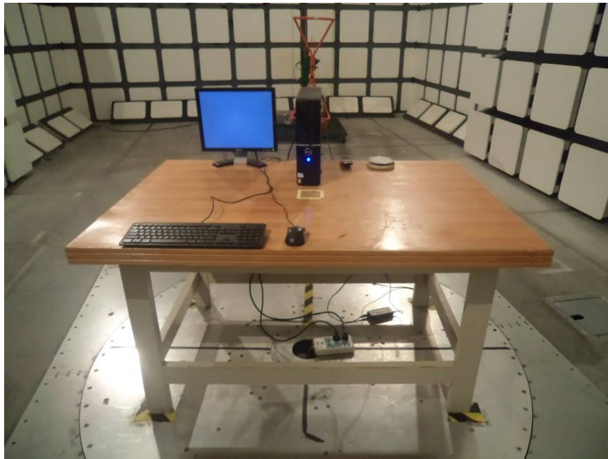
Below 1 GHz: Radiated Emissions – Front View (Downloading mode)
