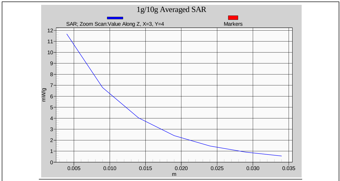
Head-Tissue-Simulating-Liquid 1950MHz
