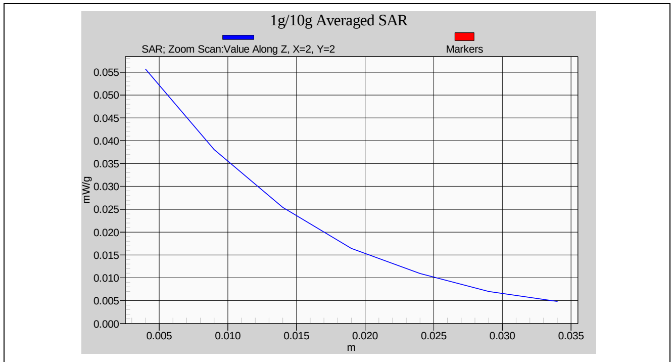
Head SAR Measurement _ Right Cheek CH4
