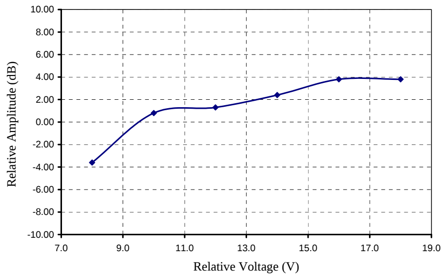
Figure 6.4. Relative emission at 135 kHz vs. supply voltage.
