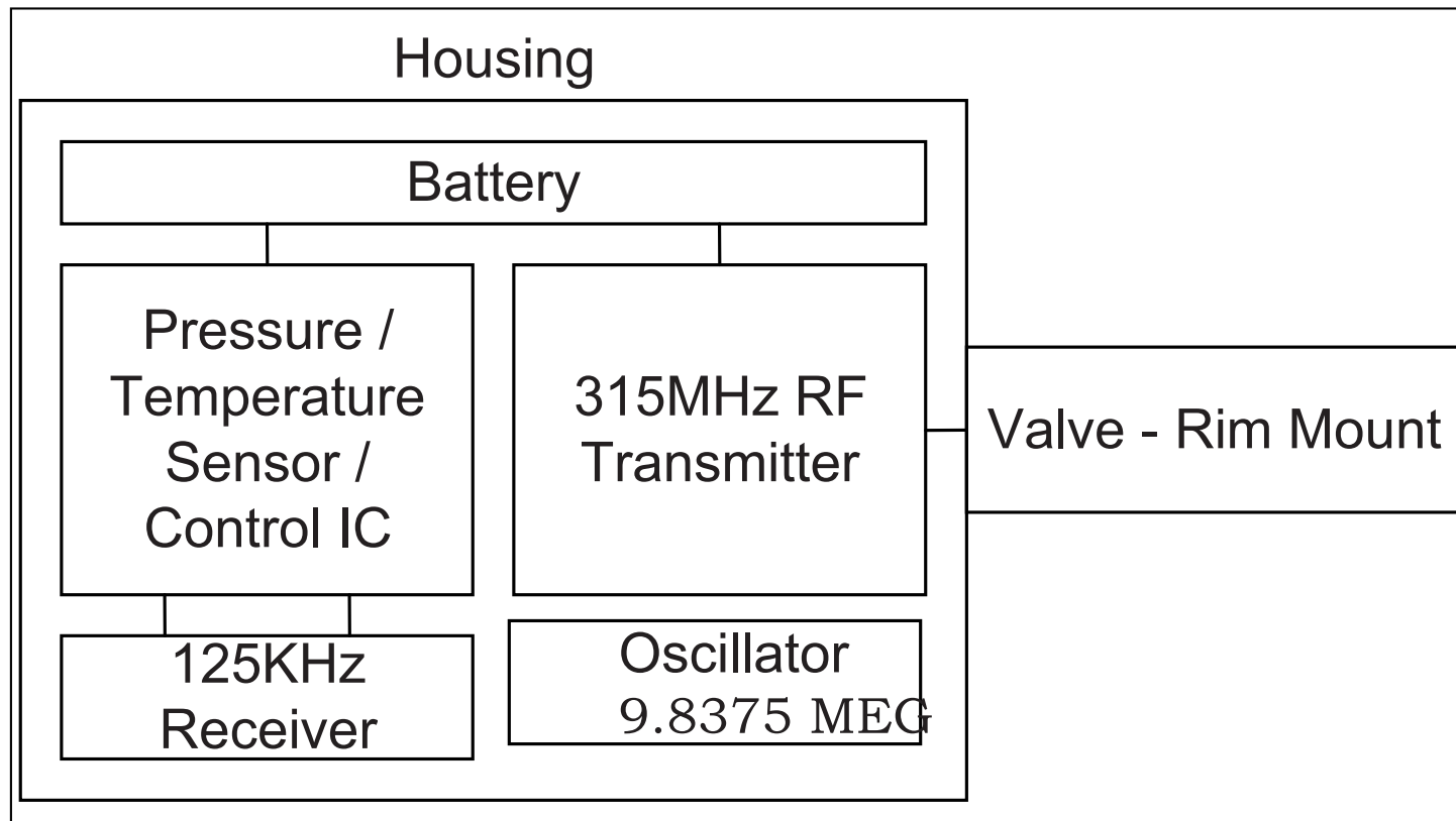
Figure 2. TPM Sensor Block Diagram
