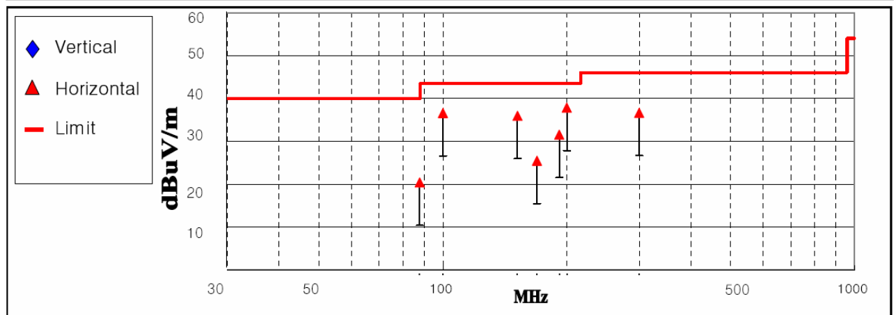
&lt; Fig 6. Radiated emission result _ Play mode &gt;
