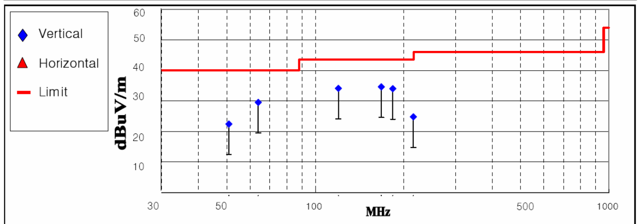
&lt; Fig 7. Radiated emission result _ AV-in mode &gt;
