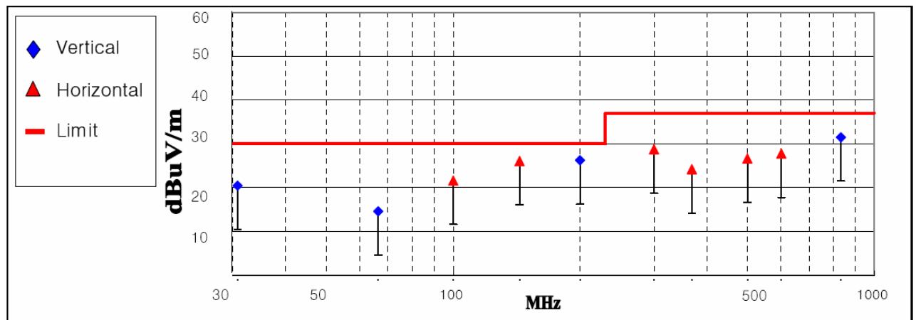
< Fig 4. Radiated emission result _ Download mode >
