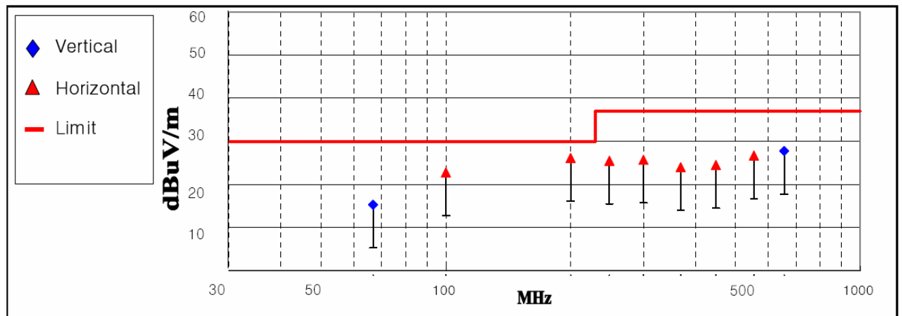
&lt; Fig 5. Radiated emission result _ Navigation mode &gt;
