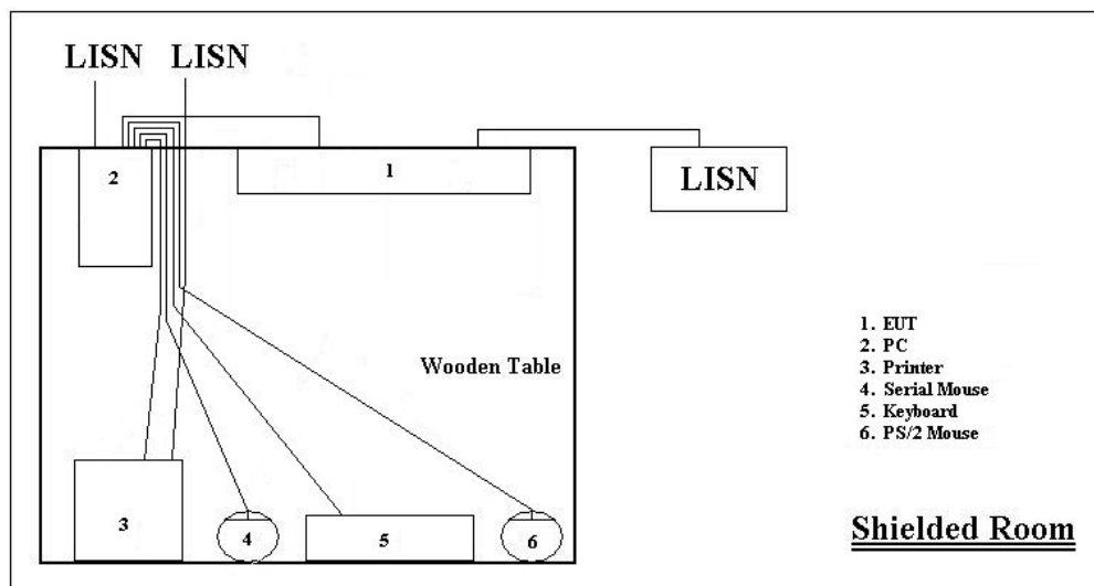
Conducted Emissions
