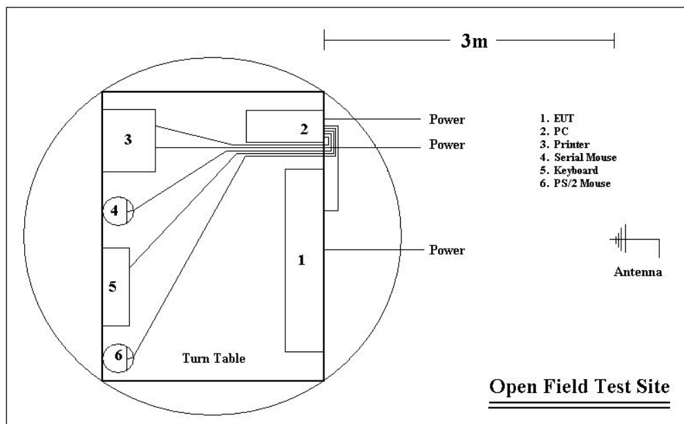
Radiated Emissions
