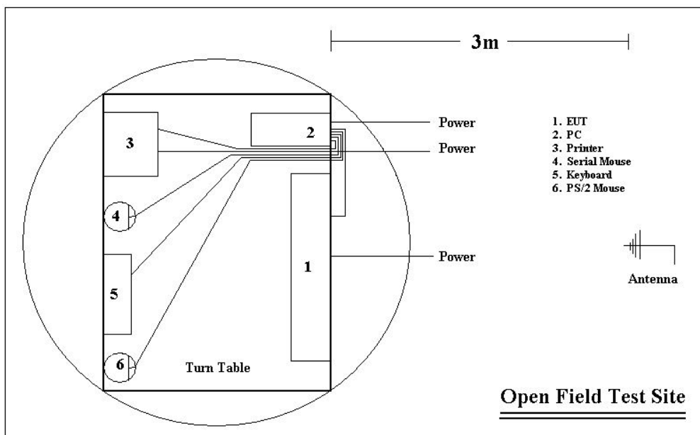
Radiated Emissions
