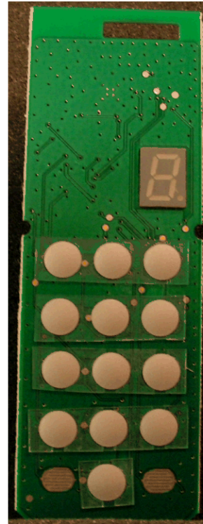
CK-MIAAA PCB – Top-Side
