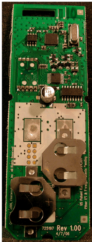
CK-MICC PCB – Bottom-Side
