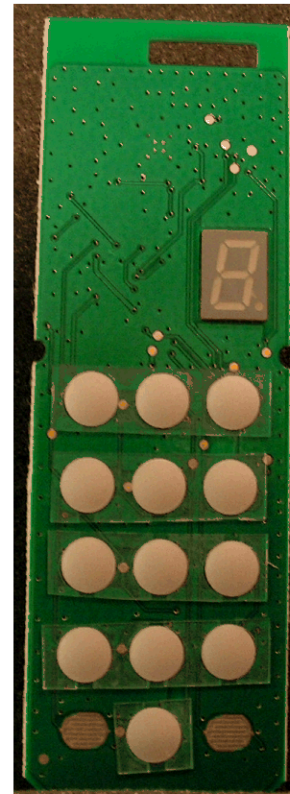
CK-MICC PCB – Top-Side
