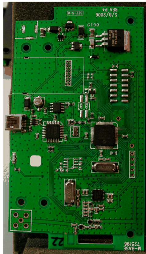
CB-500-MIU PCB – Top-Side
