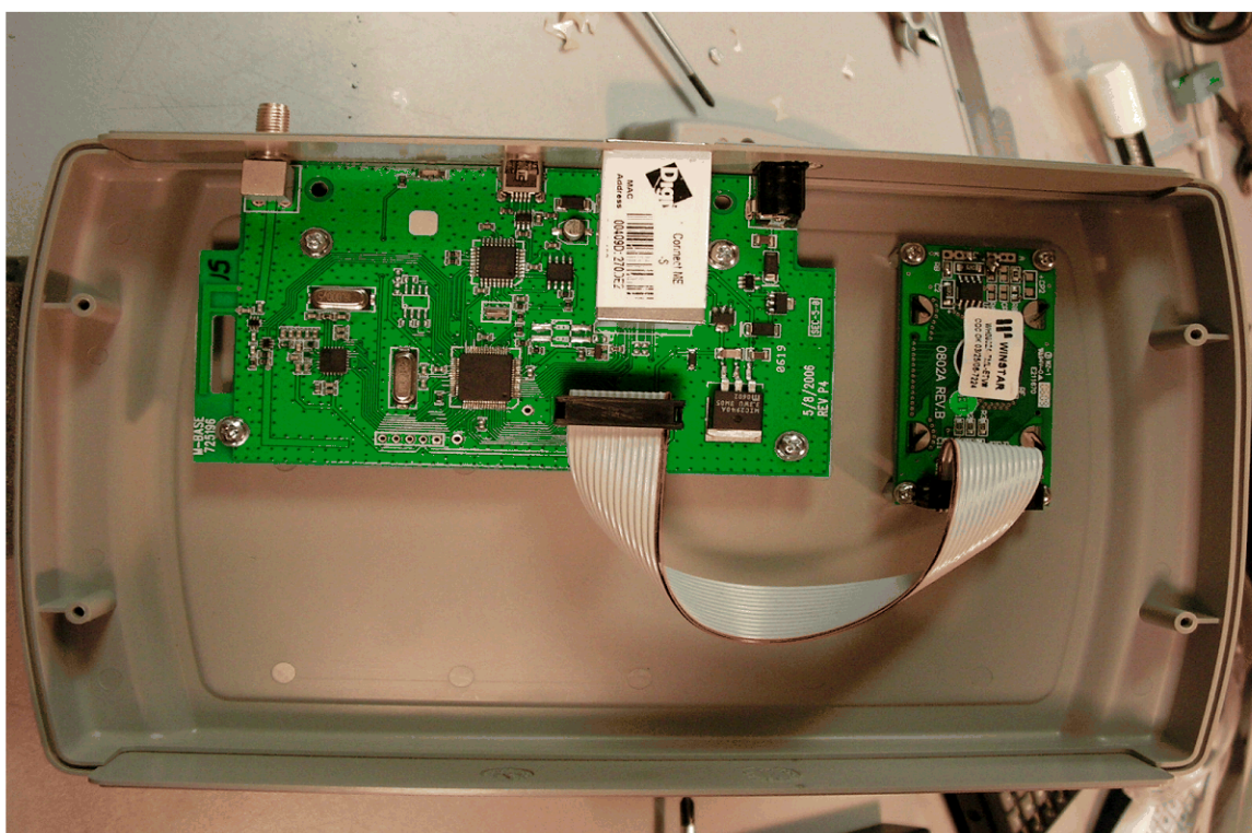
CB-500-MIE Assembly – Bottom Half of Clam-Shell
