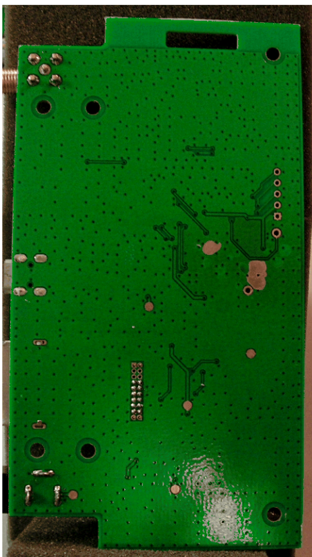
CB-500-MIE PCB – Back-Side
