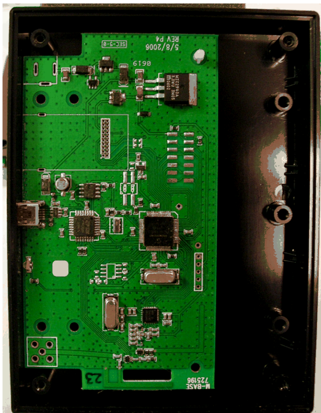
CB-500-MIU PCB – Bottom-Side
