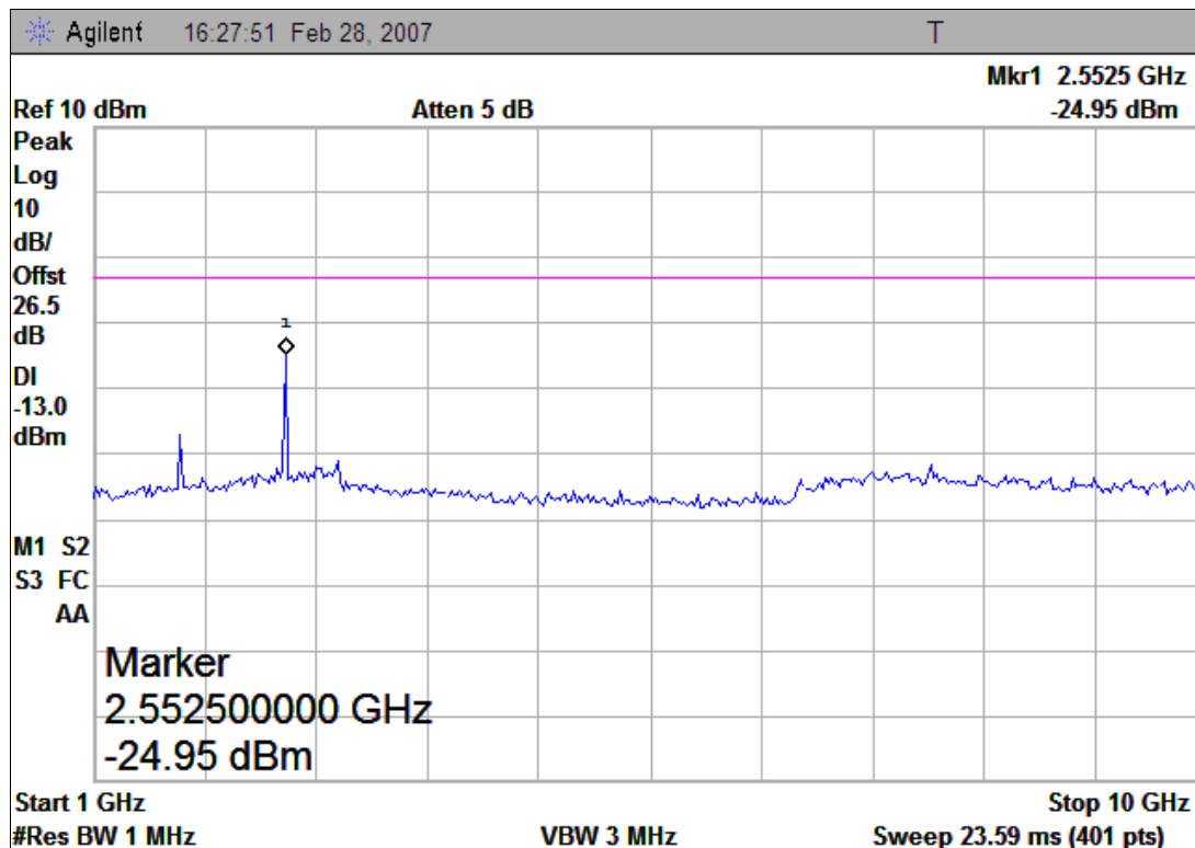
(Plot C.2: Channel = 251, 1GHz to 10GHz)
