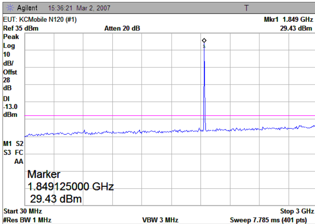
(Plot A.1: Channel = 512, 30MHz to 3GHz)
