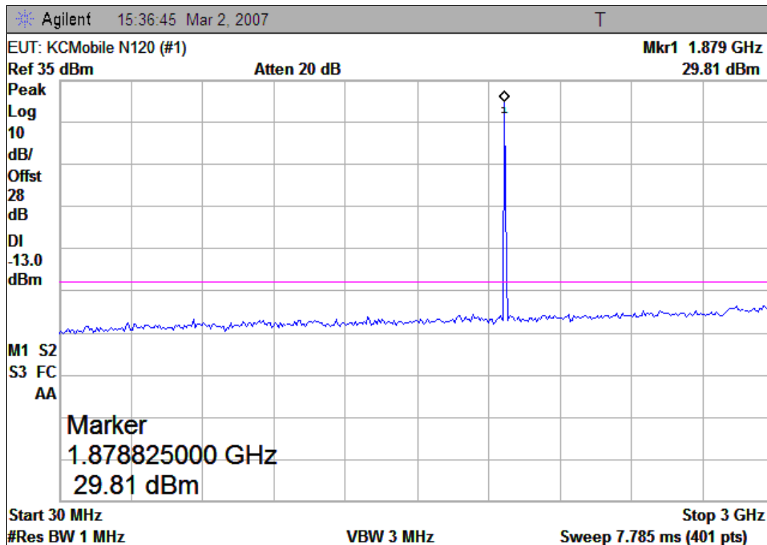
(Plot B.1: Channel = 661, 30MHz to 3GHz)
