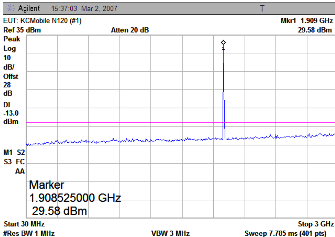
(Plot C.1: Channel = 810, 30MHz to 3GHz)
