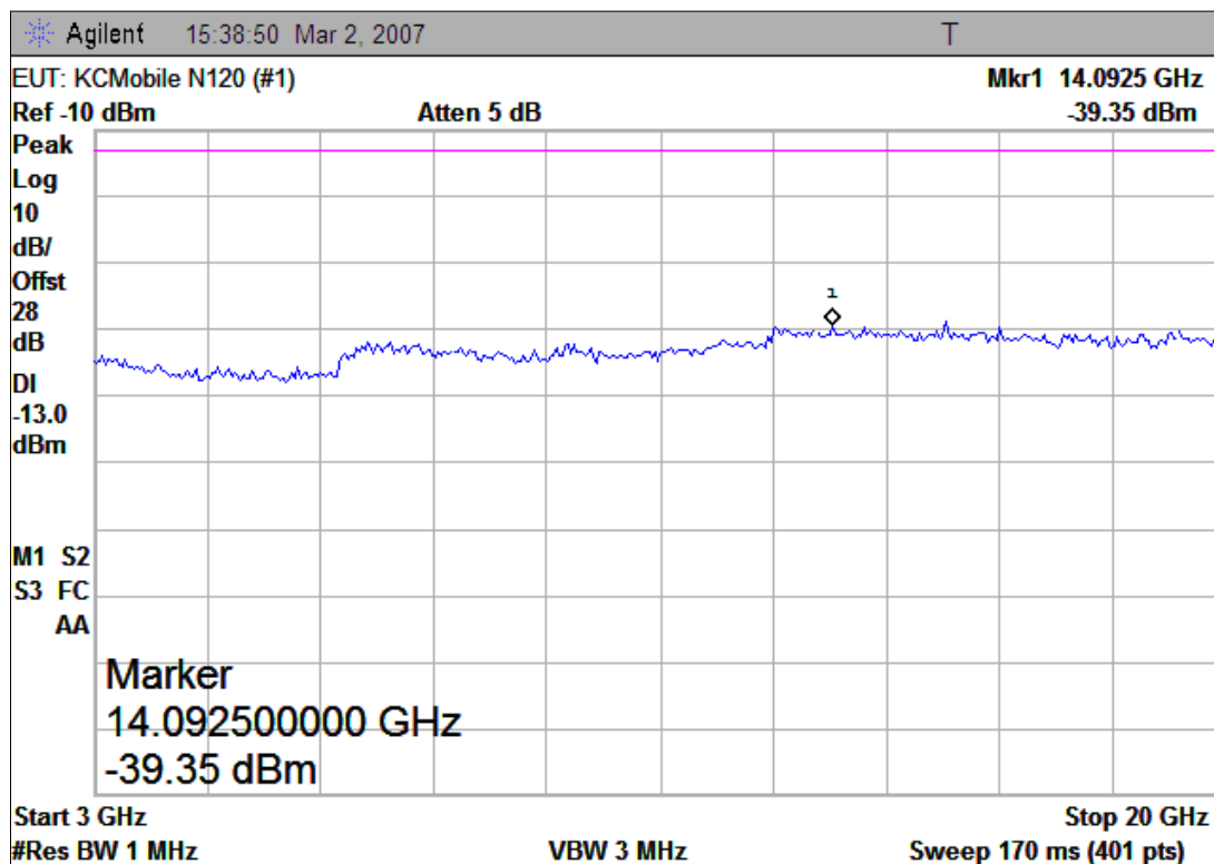
(Plot C.2: Channel = 810, 3GHz to 20GHz)
