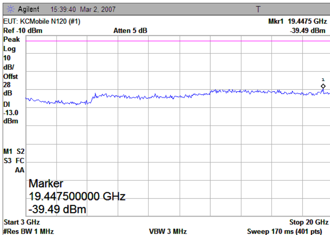
(Plot A.2: Channel = 512, 3GHz to 20GHz)
