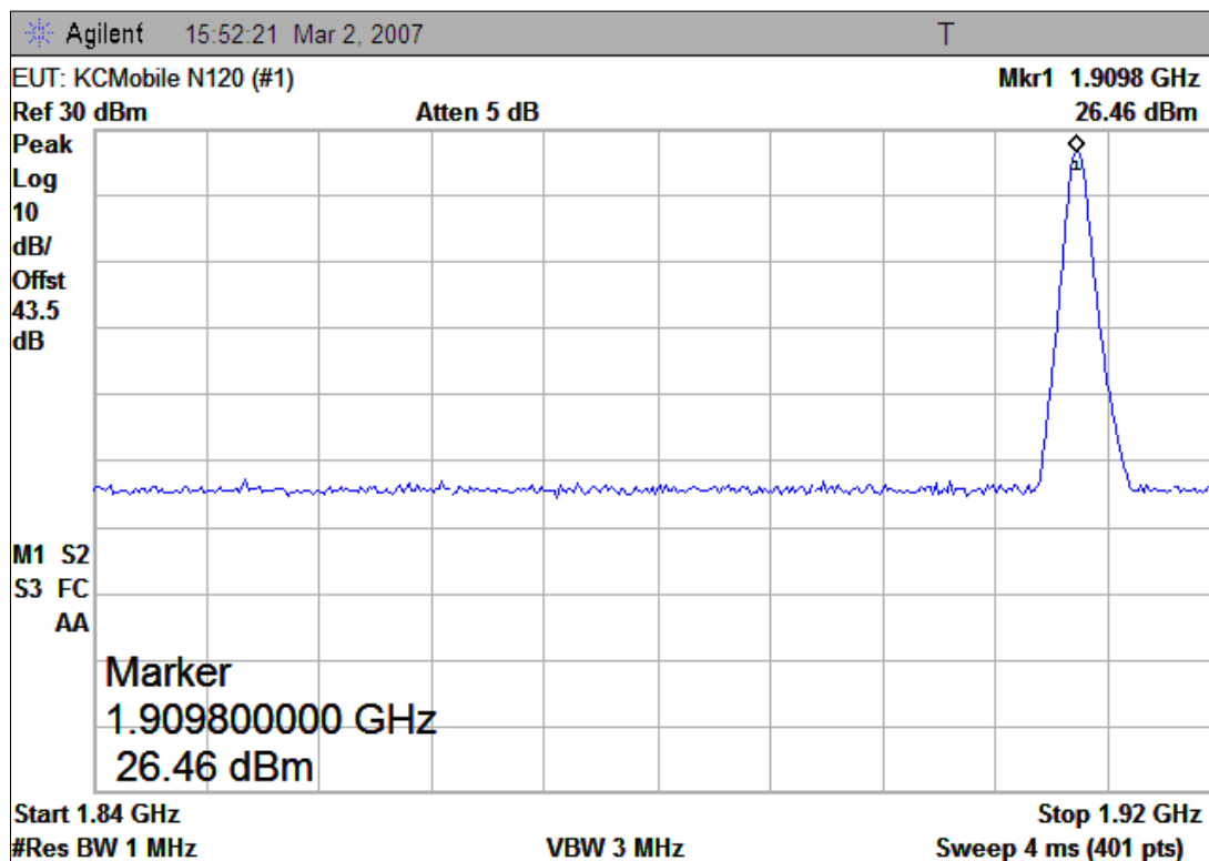
(Plot C: Channel = 810)
