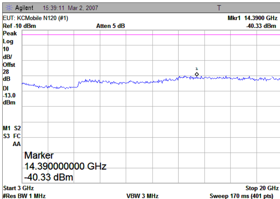
(Plot B.2: Channel = 661, 3GHz to 20GHz)
