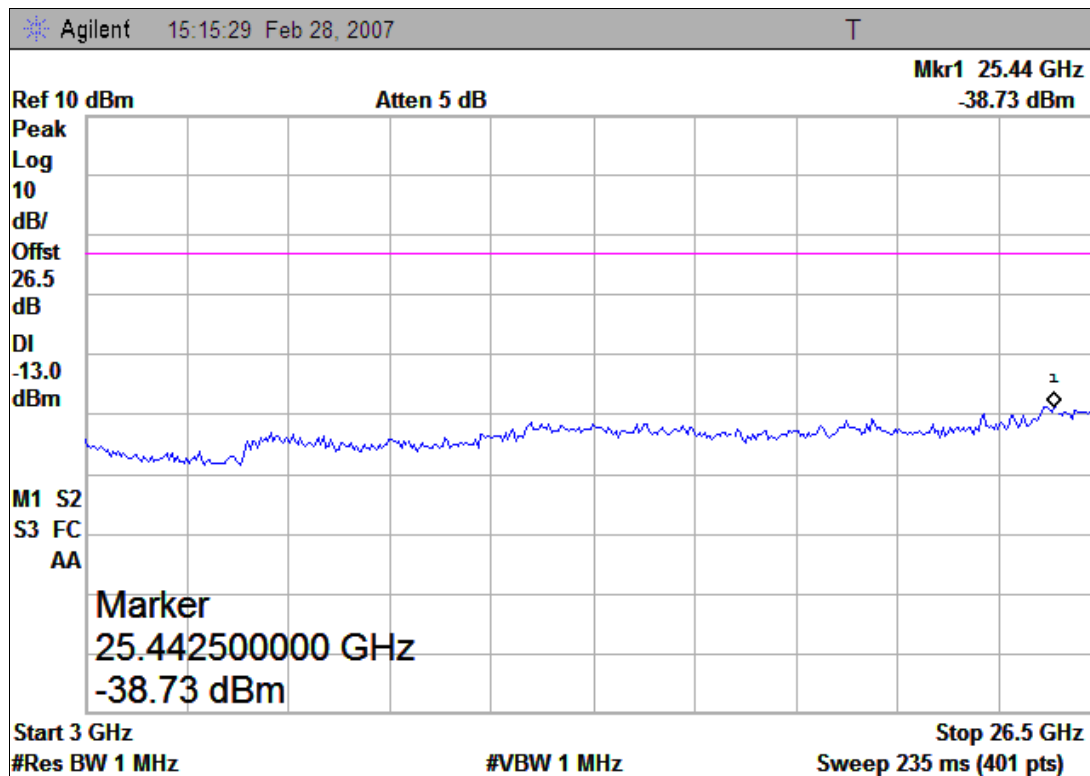
(Plot B.2: Channel = 661, 3GHz to 26.5GHz)
