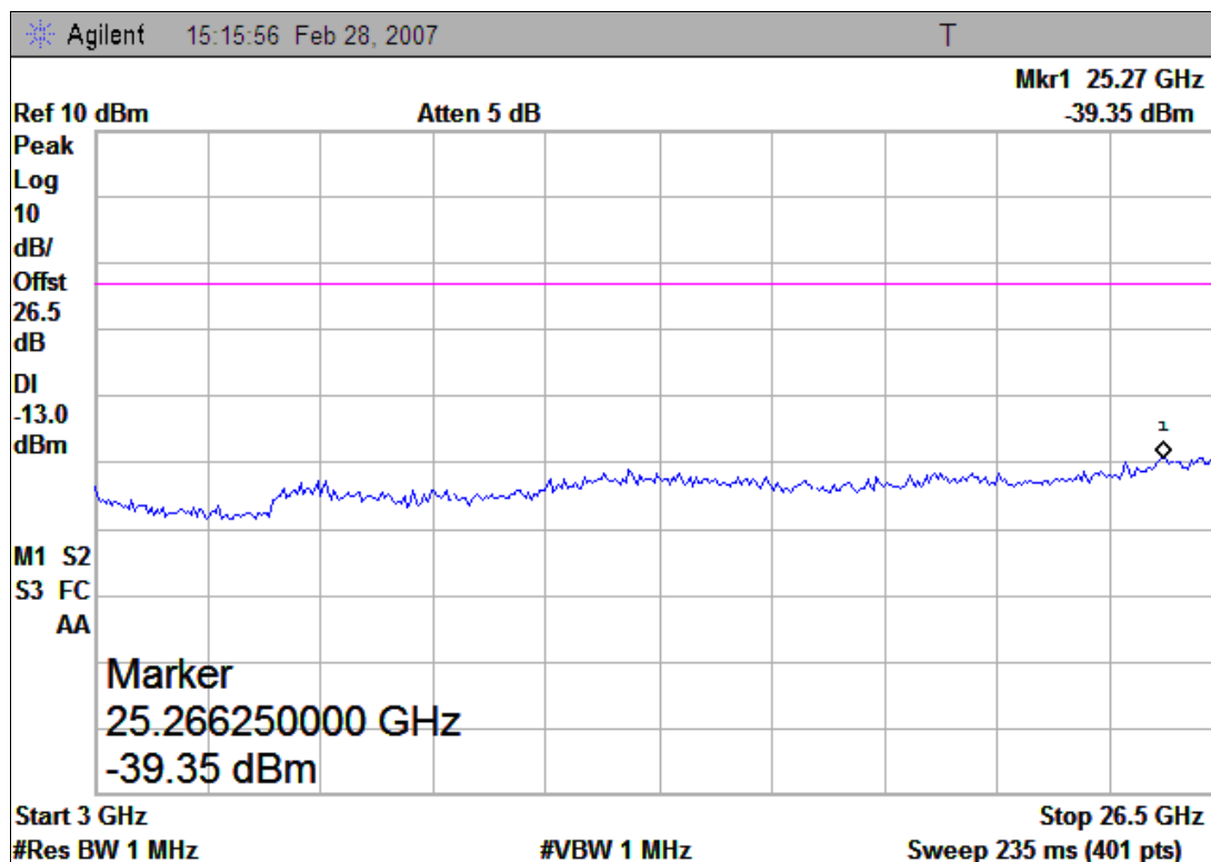
(Plot A.2: Channel = 512, 3GHz to 26.5GHz)
