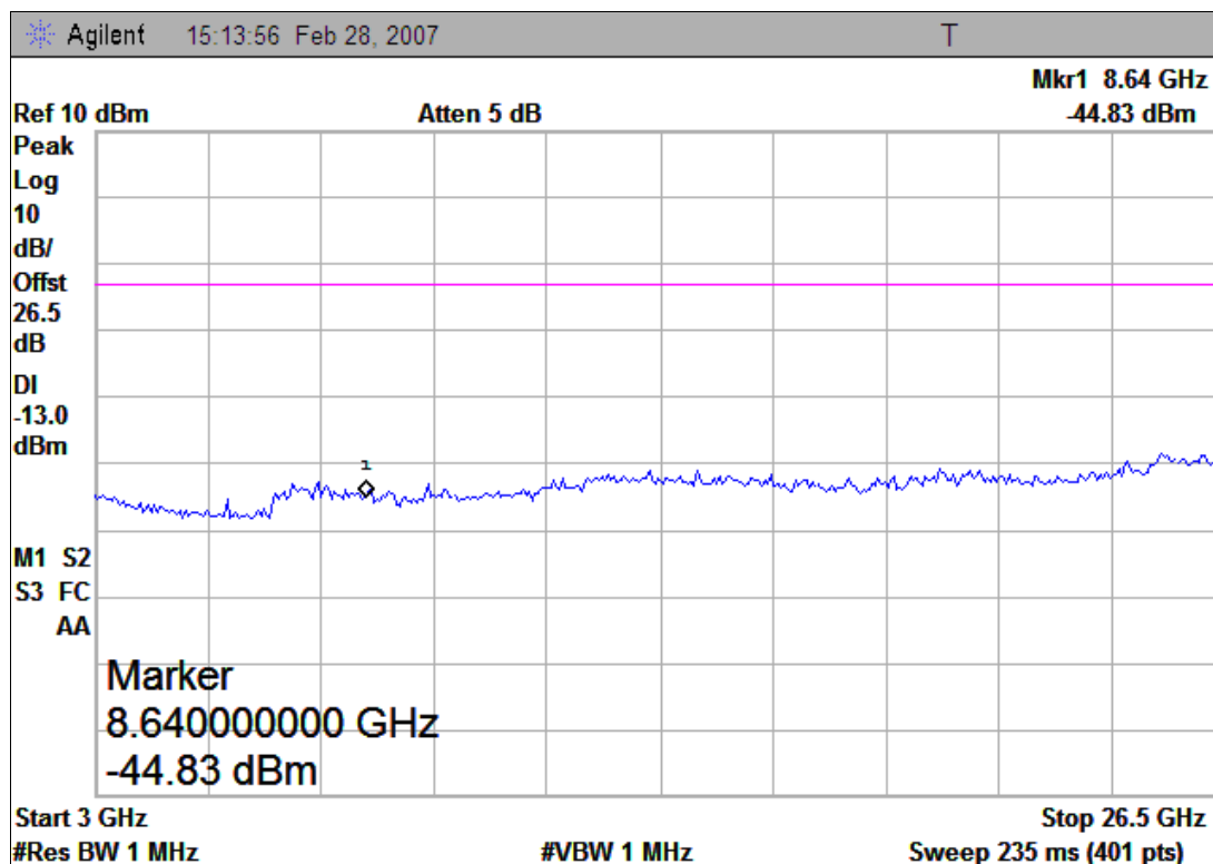
(Plot C.2: Channel = 810, 3GHz to 26.5GHz)
