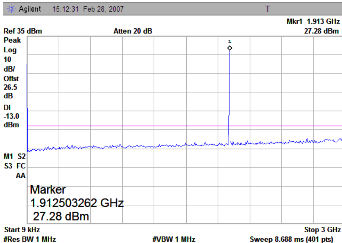
(Plot C.1: Channel = 810, 9kHz to 3GHz)
