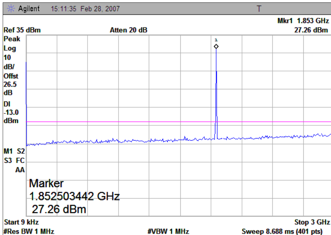
(Plot A.1: Channel = 512, 9kHz to 3GHz)
