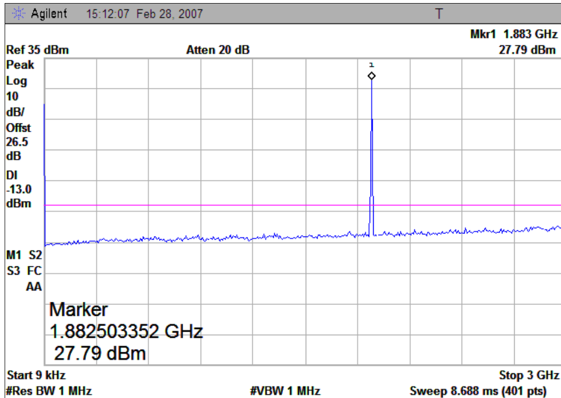
(Plot B.1: Channel = 661, 9kHz to 3GHz)
