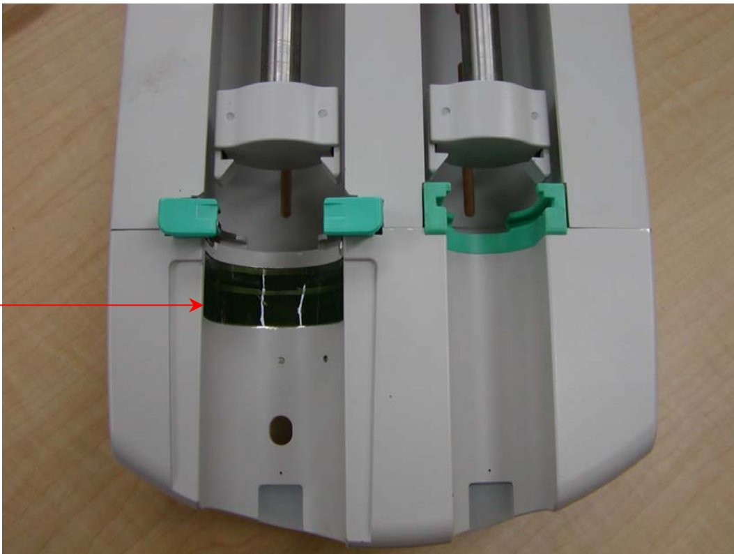
Antenna Location
