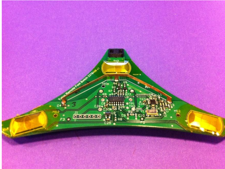
Figure 1 - Internal Photos
