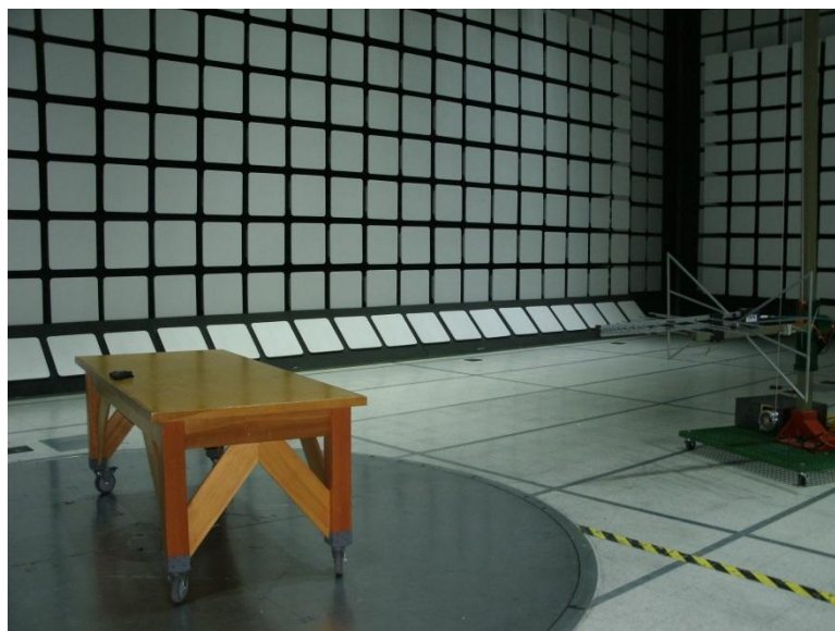
Figure 2 - Test Setup Photos
