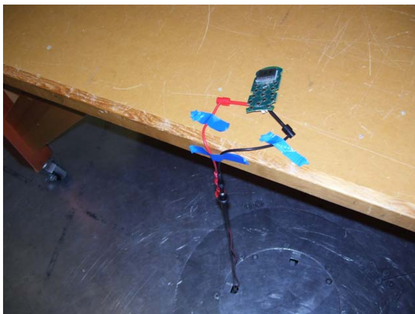
Figure 4 - Radiated Emissions Testing, 1 - 26GHz, Horizontal
