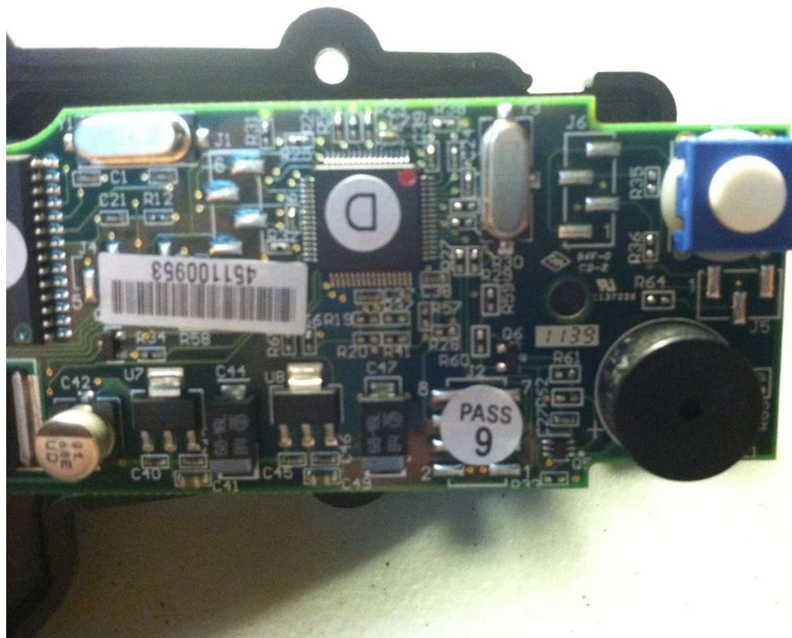
Figure 7 - RF Board, detail
