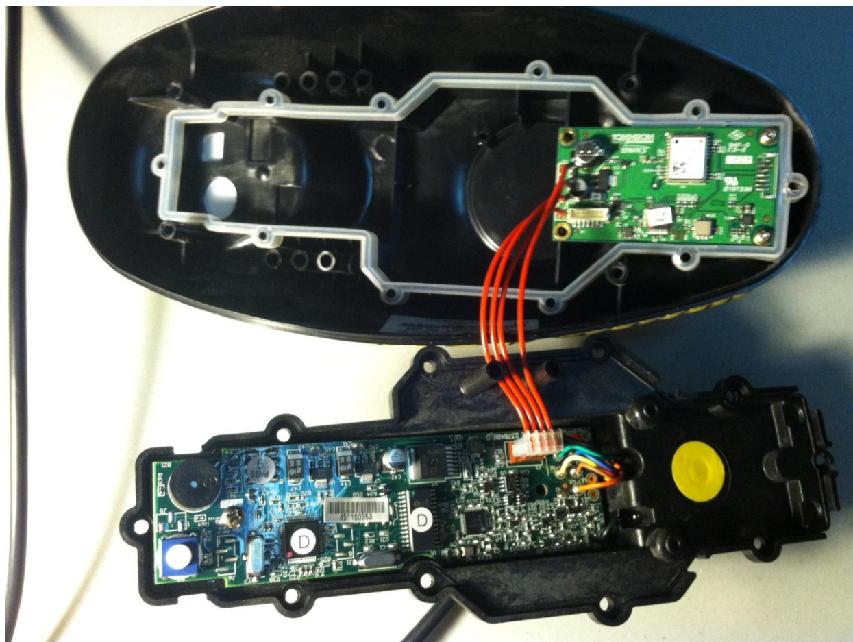
Figure 2 - Cover disconnected
