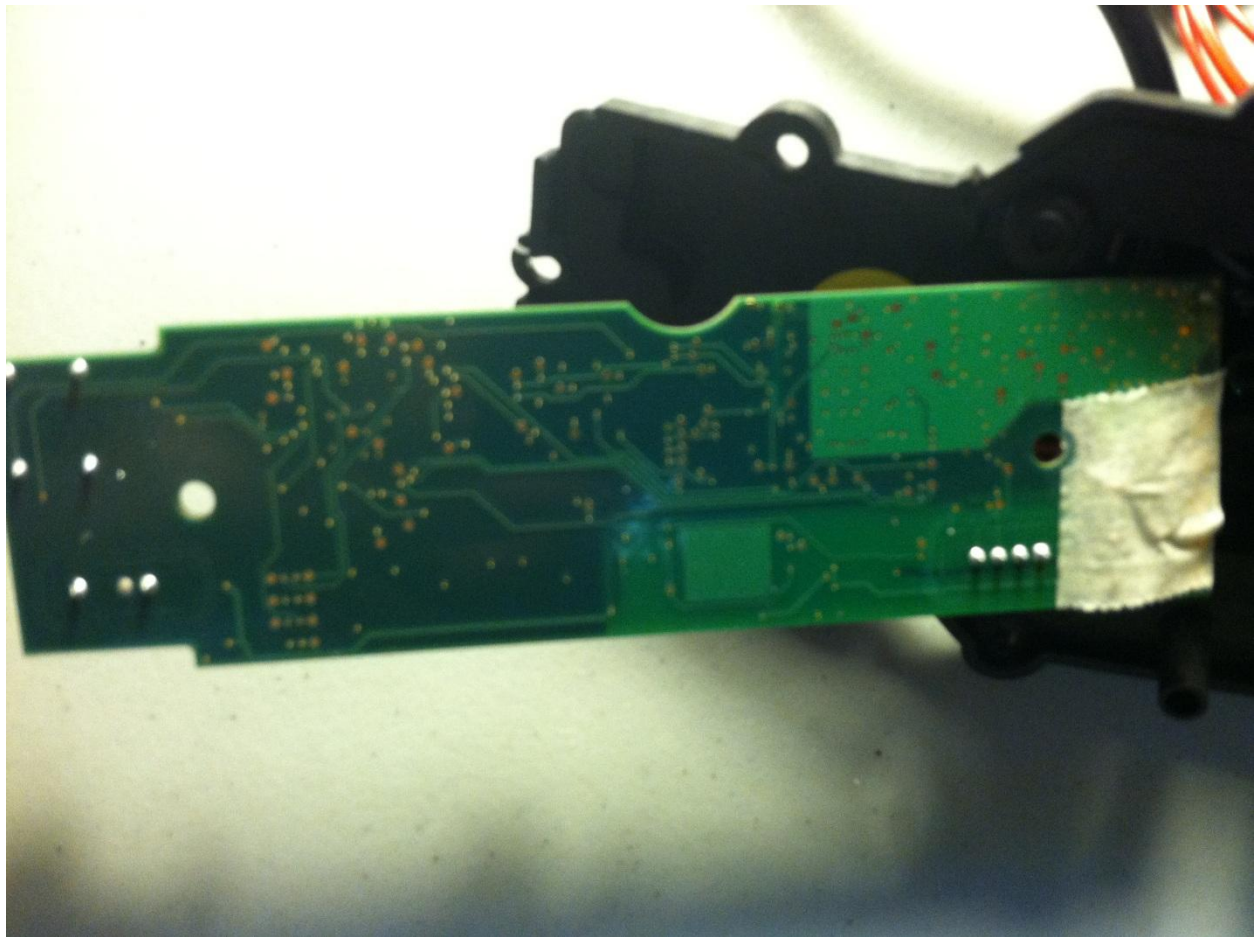
Figure 4 - RF Board, bottom
