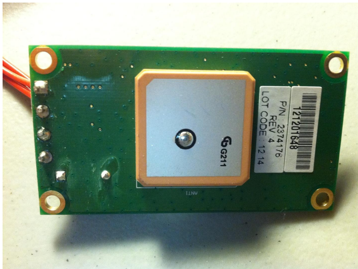
Figure 6 - Compass/combination board, bottom. GPS antenna
