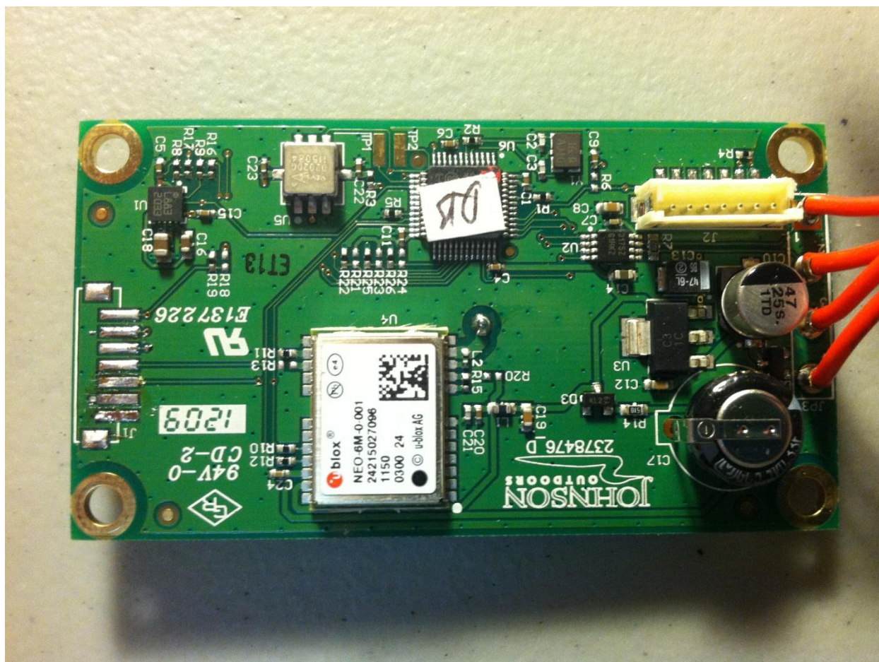
Figure 5 - Compass/combination board
