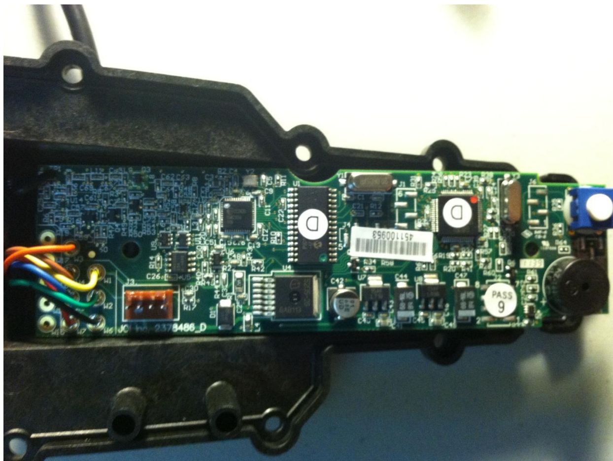
Figure 3 - RF board detail – black wire in bottom left is the antenna.
