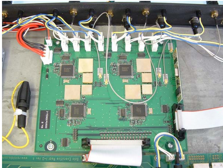
CLOSE UP OF RF PCB
