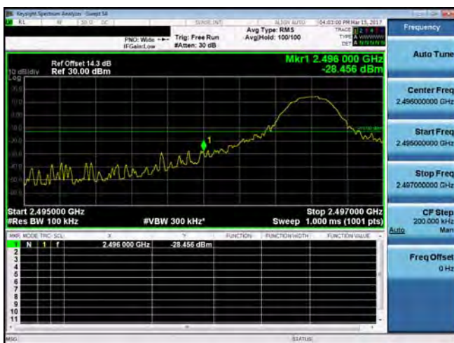
Band Edge_Band41_10MHz_QPSK_1_0_LowCH39700
