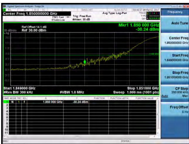
Band Edge_Band2_20MHz_QPSK_1_0_LowCH18700-1860
