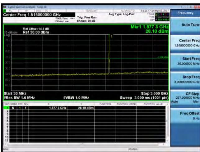
30MHz-3GHz_Band2_10MHz_QPSK_1_0_MidCH18900-1880
