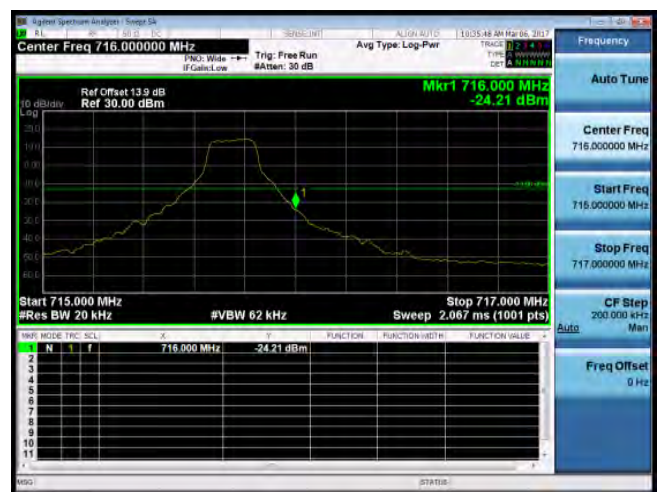
Band Edge_Band12_1.4MHz_QPSK_1_5_HighCH23173-715.3
