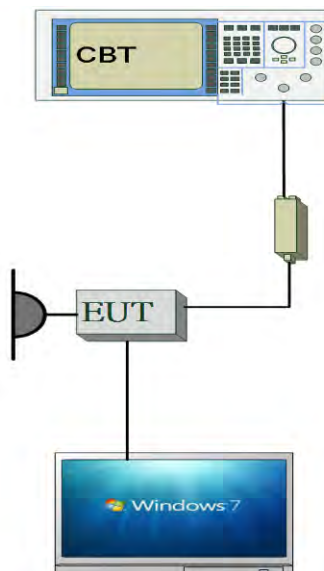
Fig. 2-2 AC Power Line Conducted Emission
