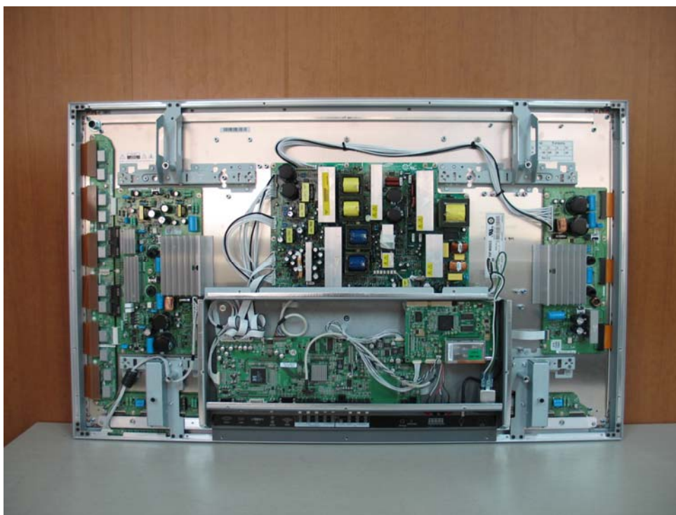
Inner View
