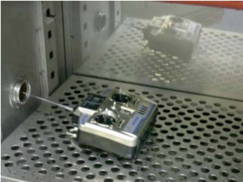
Frequency Stability Test Setup
