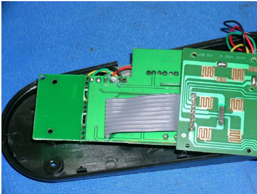
Product Main PCB solder side (View 2)
