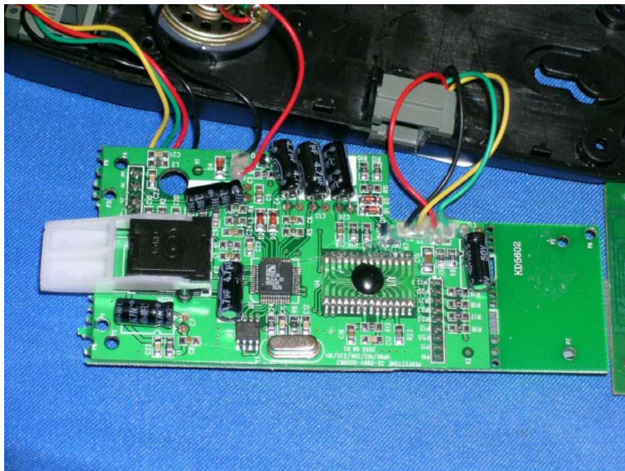
Product Main PCB comp side
