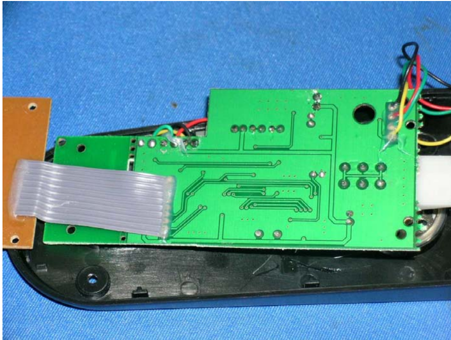
Product Main PCB solder side (View 1)
