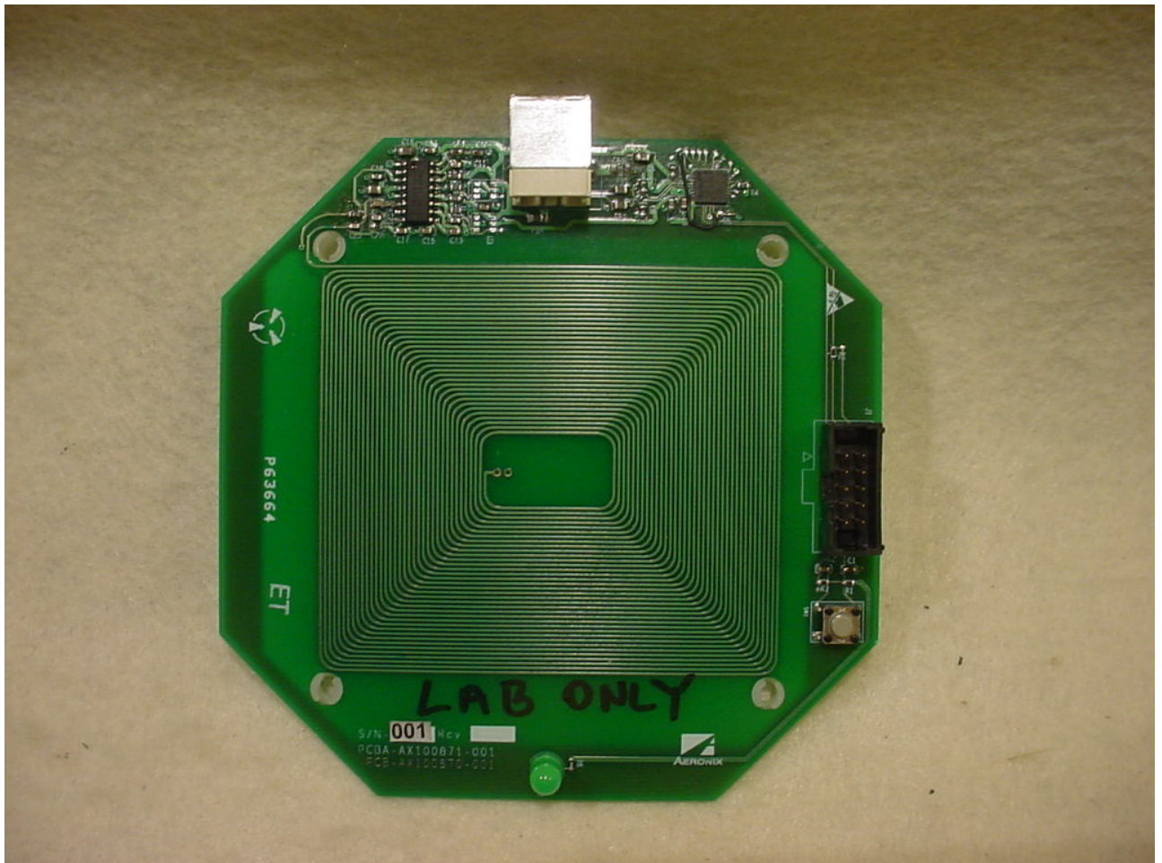
Figure 2: RF PCB - Top View
