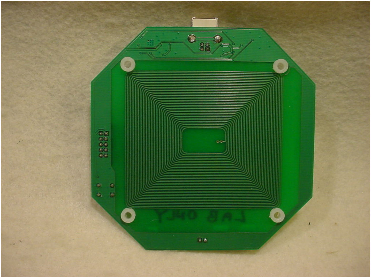
Figure 3: RF PCB – Bottom View
