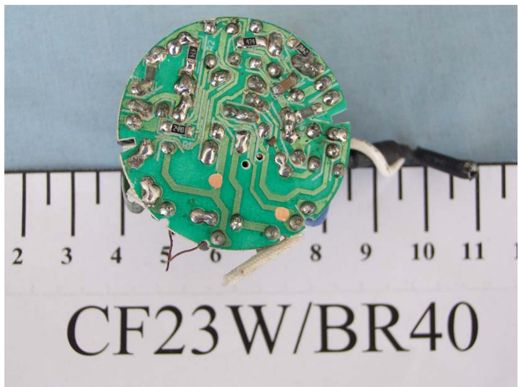
FIGURE 20 COMPACT FLUORESCENT LAMP (M/N: CF 23W/BR40) MAIN BOARD (SOLDERED SIDE)
