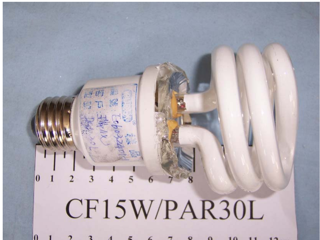
FIGURE 1 COMPACT FLUORESCENT LAMP (M/N: CF 15W/PAR30L) LAMP SHADE REMOVED
