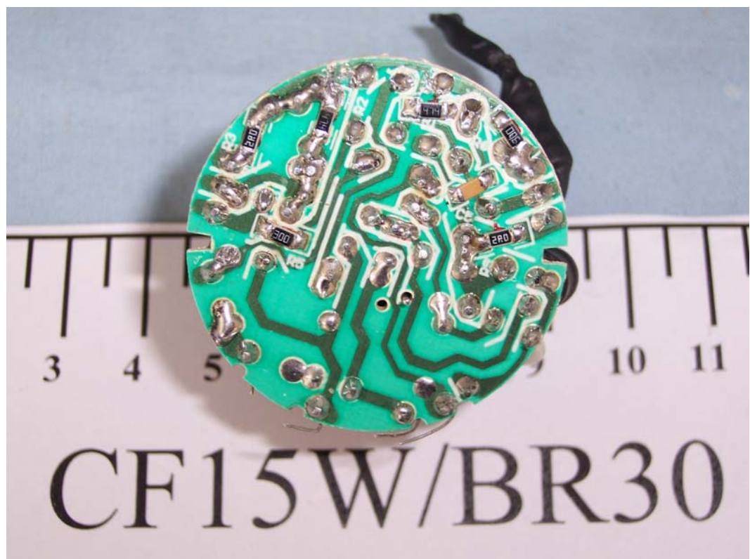
FIGURE 8 COMPACT FLUORESCENT LAMP (M/N: CF 15W/BR30) MAIN BOARD (SOLDERED SIDE)
