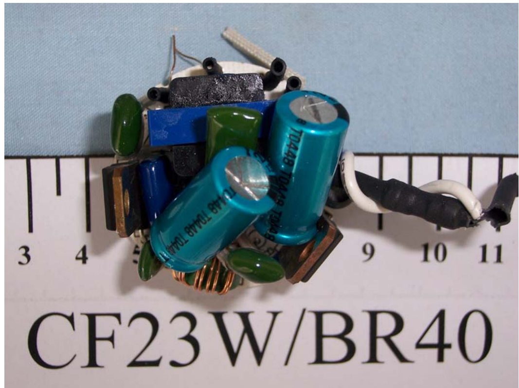
FIGURE 19 COMPACT FLUORESCENT LAMP (M/N: CF 23W/BR40) MAIN BOARD (COMPONENT SIDE)
