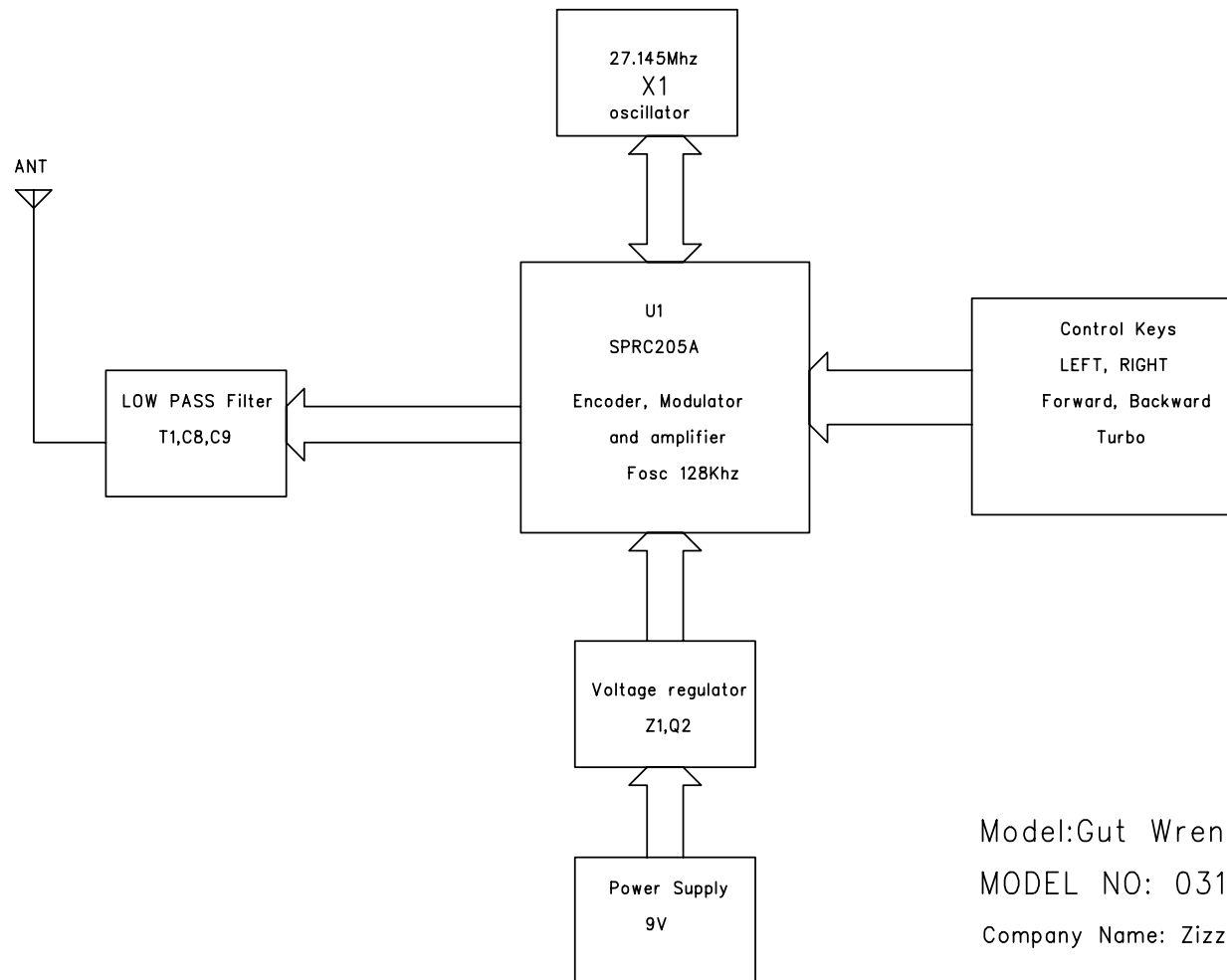
TX 27.145MhzMhz Block Diagram of Gut Wrencher
