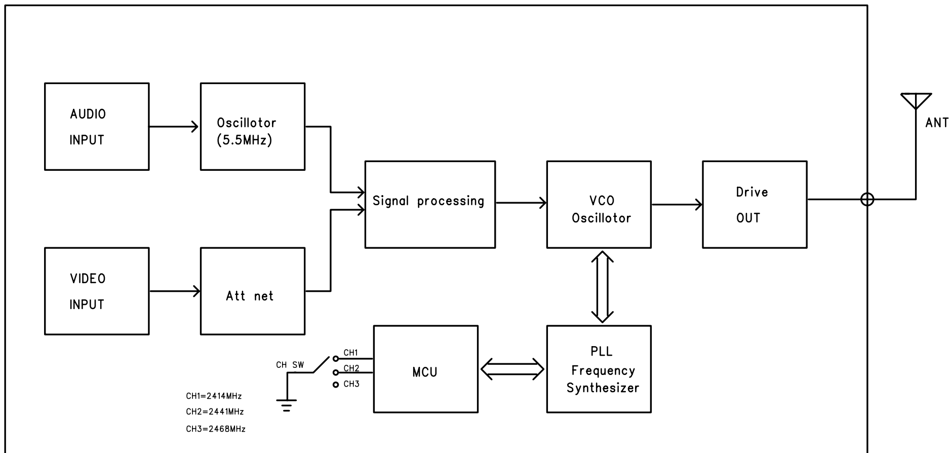
SB0001 Transmitter block diagram
