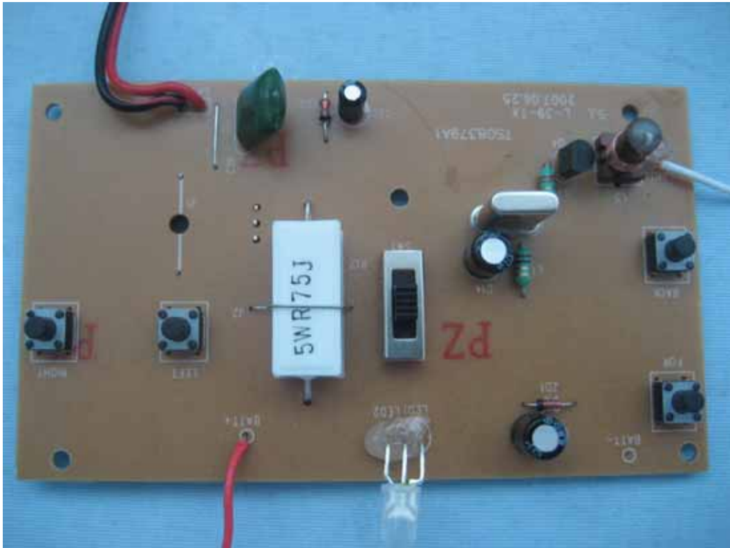
TOP VIEW OF INTERNAL PHOTO
