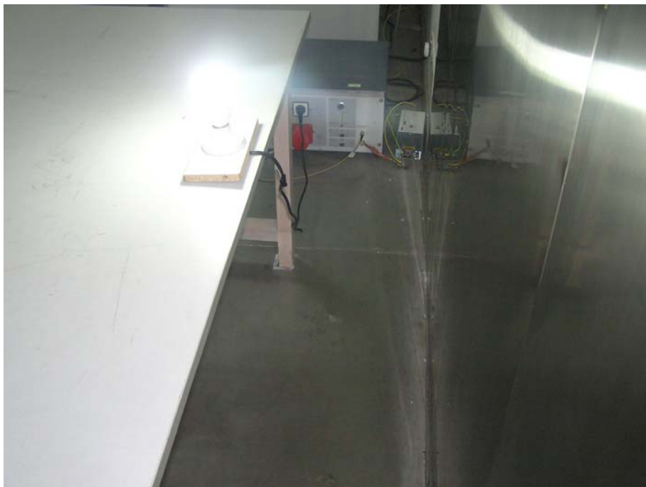
G-9W: Conducted Emission - Rear View
