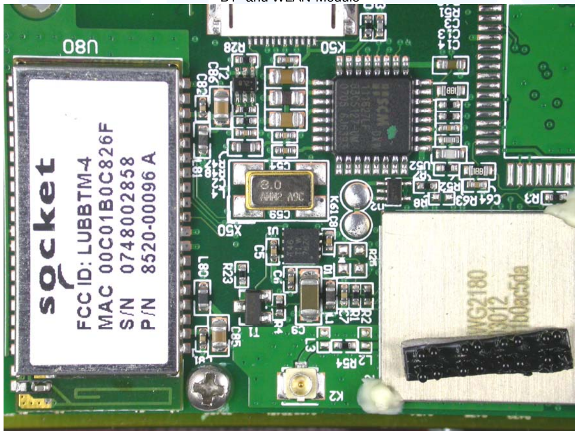
BT- and WLAN-Module
