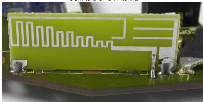
GSM and GPS-Antenna
