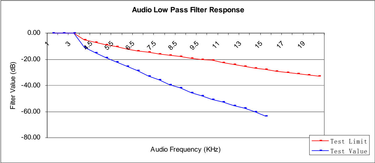
Response for 25.0 KHz Channel Separation
