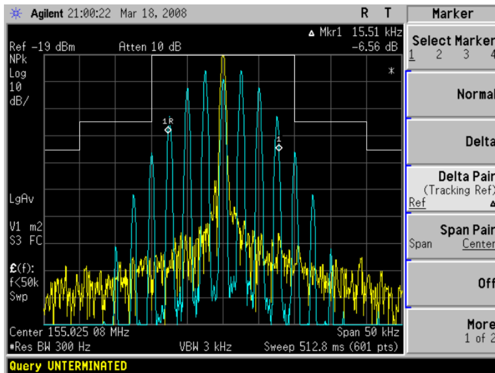
The Worst Emission Mask for 25 KHz channel Separation
