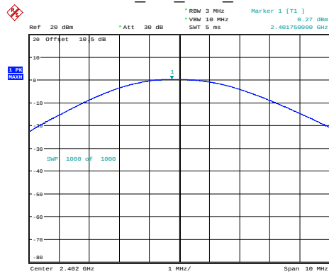
BLE_1M_Low_Channel
