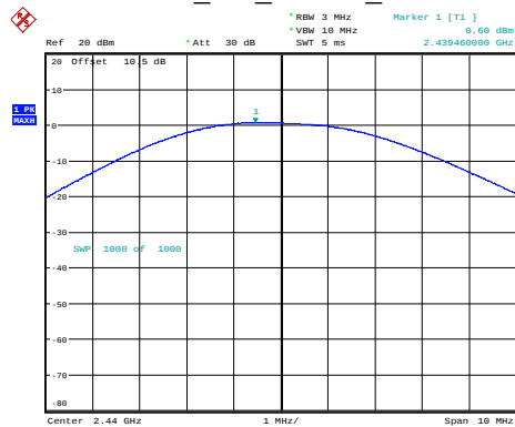
BLE_2M_Middle_Channel
