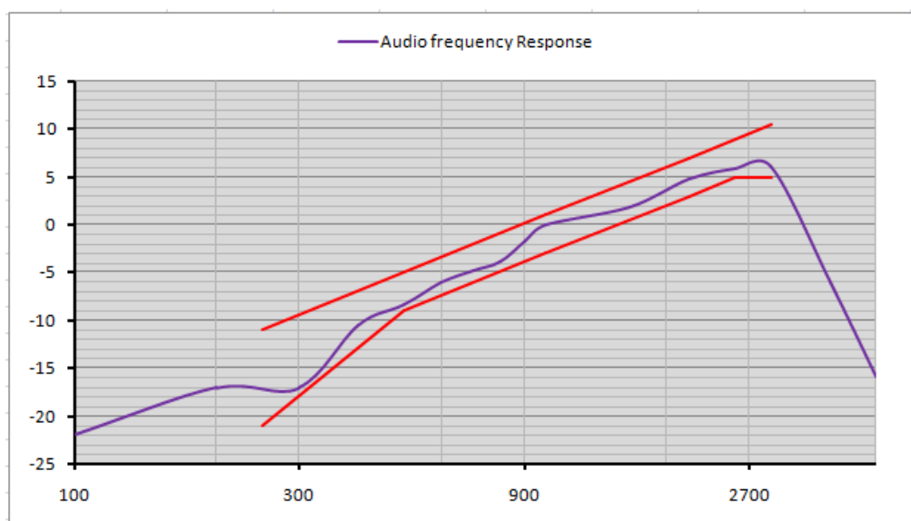
Plot B3 : 155.025MHz @ 12.5 KHz Channel Separations
