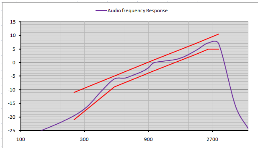
Plot B4 : 440.025MHz @ 12.5 KHz Channel Separations
