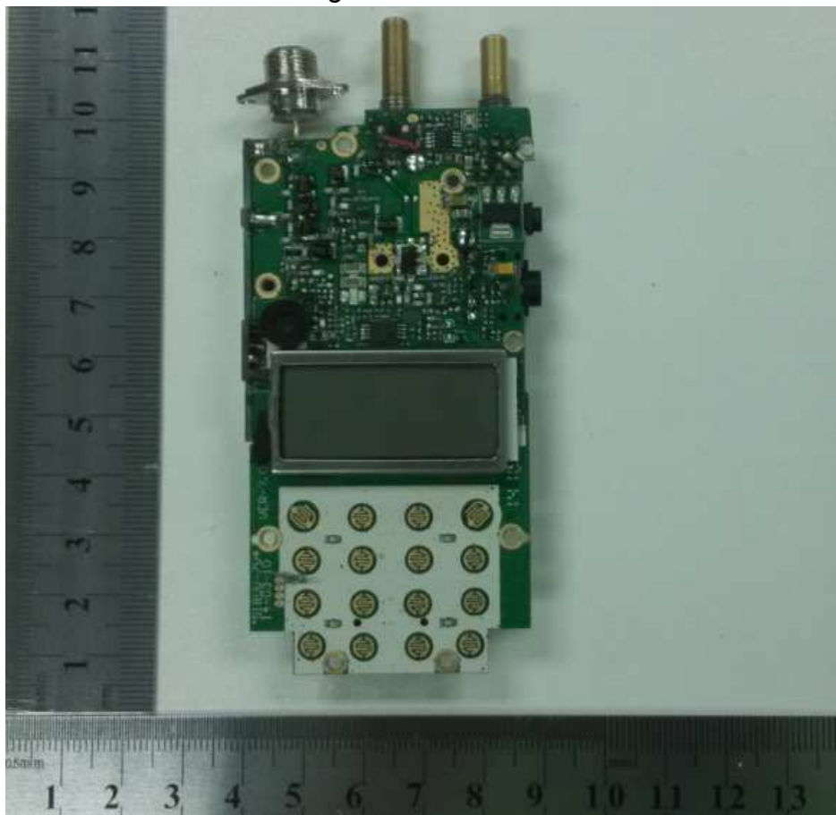
5. Mainboard front view without shielding
