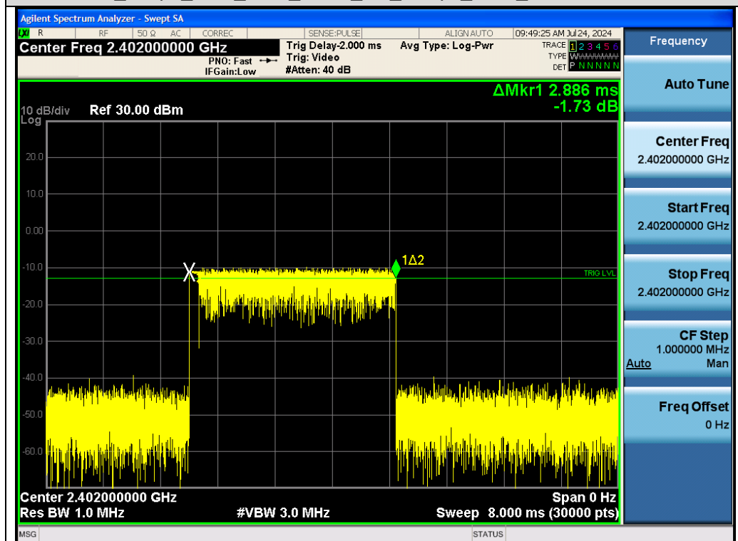
Test Graph EDR HOP ANT1 NA 3Mbps 2402 Time per Burst
