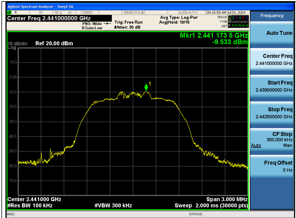
Test_Graph_EDR_ANT1_2441_2Mbps_Reference Level
