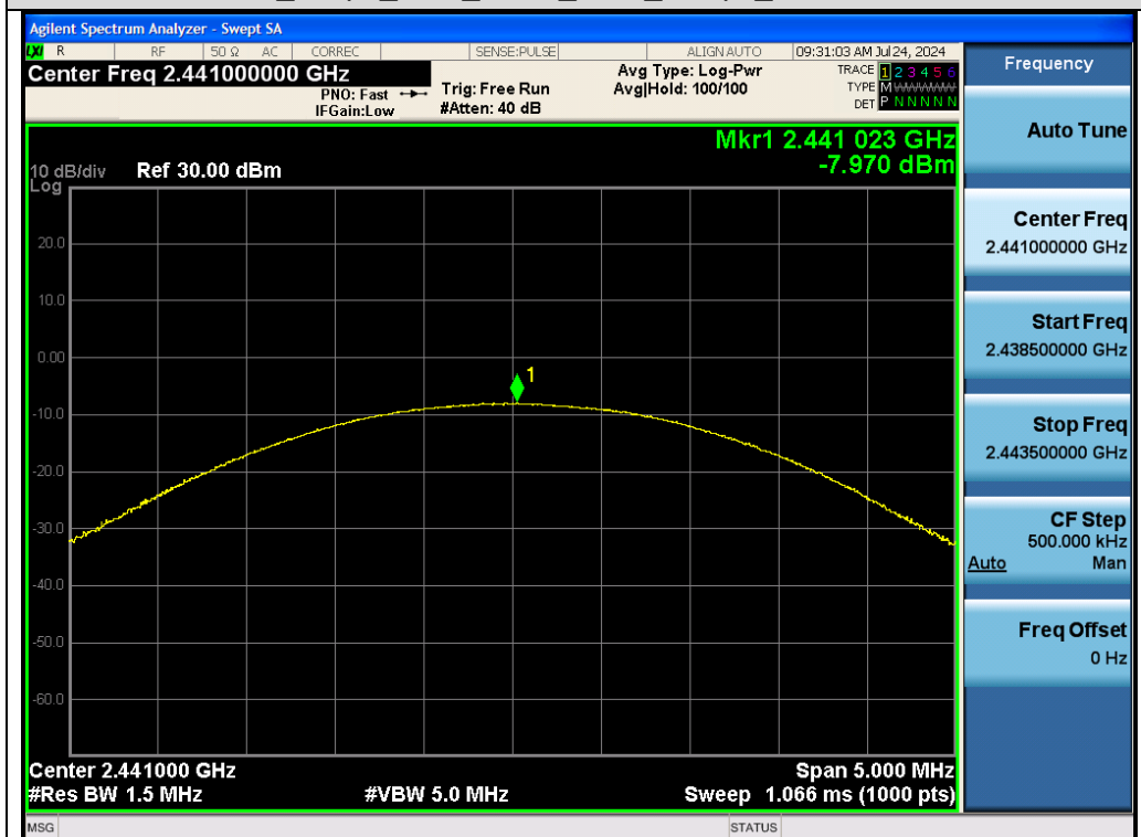
Test_Graph_EDR_ANT1_2441_3Mbps_Peak Power
