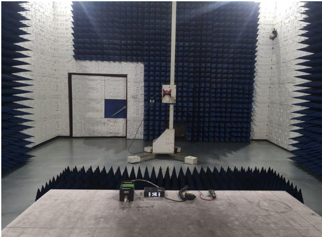
RADIATED EMISSION TEST SETUP-ABOVE 1GHZ
