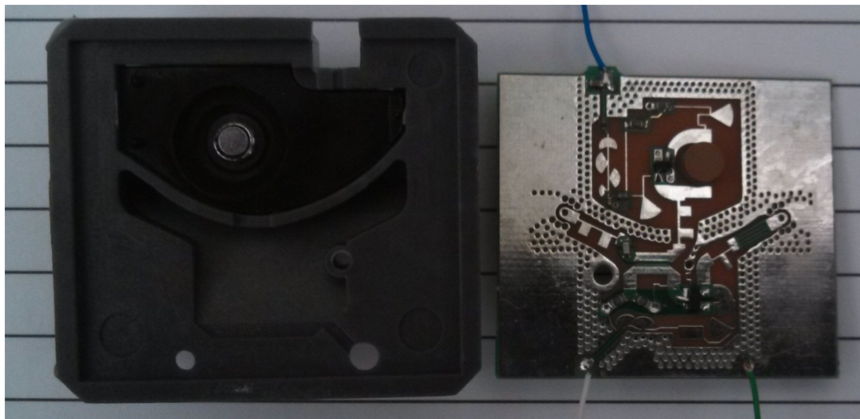
Figure 4 – Internal Photo of EUT back side of antenna board
