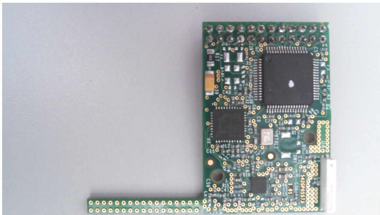
Figure 6 – Internal Photo of EUT
