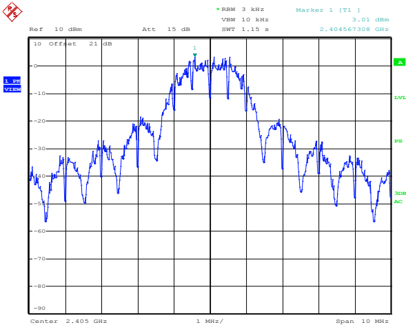
Figure 8.4-1: PSD (2405 MHz)
