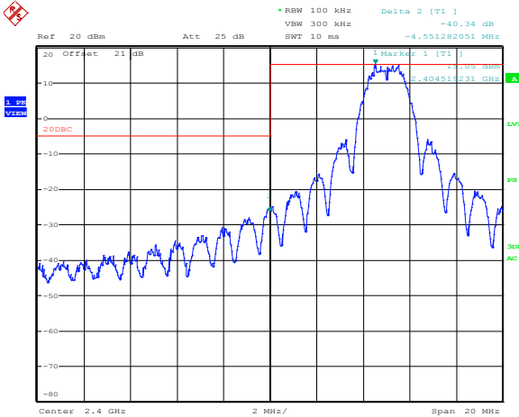
Figure 8.3-6: Lower band edge, Conducted (TX 2405 MHz)
