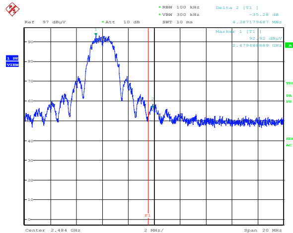
Plot 8.3-16: Upper band edge 100 kHz RBW, 300 kHz VBW, Radiated (TX 2480 MHz) – Inverted F Antenna
