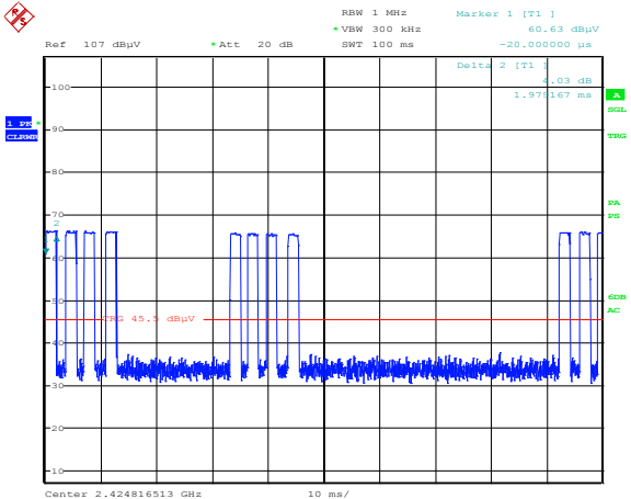
Plot 8.3-10: Measured duty cycle
