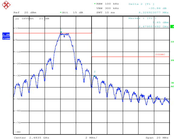
Figure 8.3-9: Upper band edge, Conducted (TX 2480 MHz) @ -12 dBm
