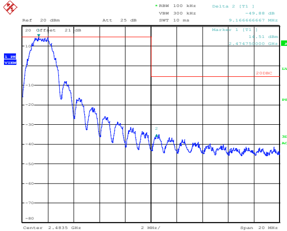
Figure 8.3-7: Upper band edge, Conducted (TX 2475 MHz)
