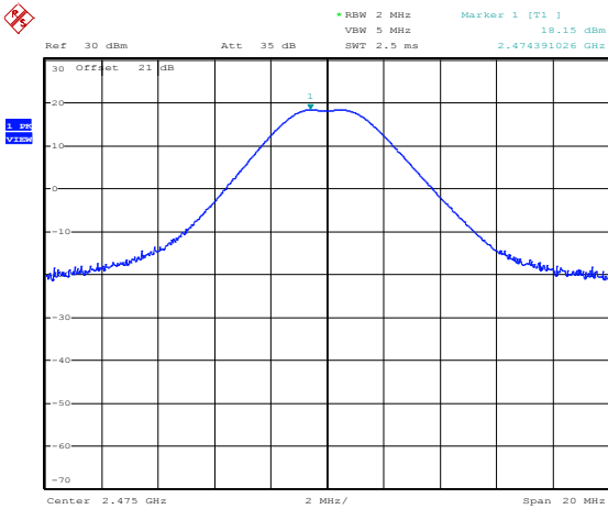
Figure 8.2-3: Conducted output power (2475 MHz)
