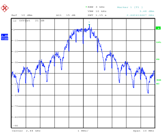
Figure 8.4-2: PSD (2440 MHz)
