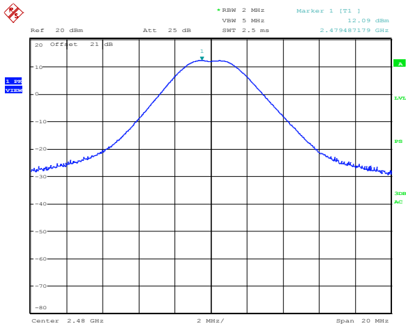
Figure 8.2-5: Conducted output power (2480 MHz) @ -12 dBm
