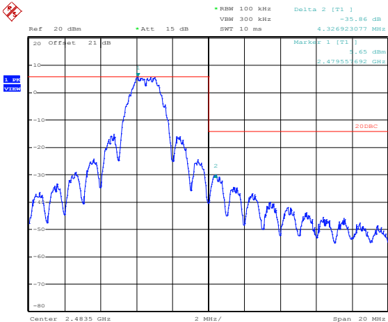
Figure 8.3-8: Upper band edge, Conducted (TX 2480 MHz) @ -14 dBm
