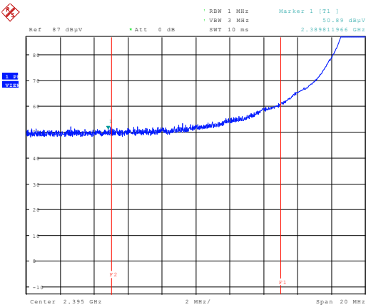
Figure 8.3-13: Lower band edge, Radiated (TX 2405 MHz) – Circular SEMI-Loop Antenna
