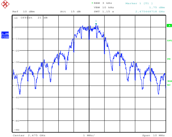
Figure 8.4-3: PSD (2475 MHz)
