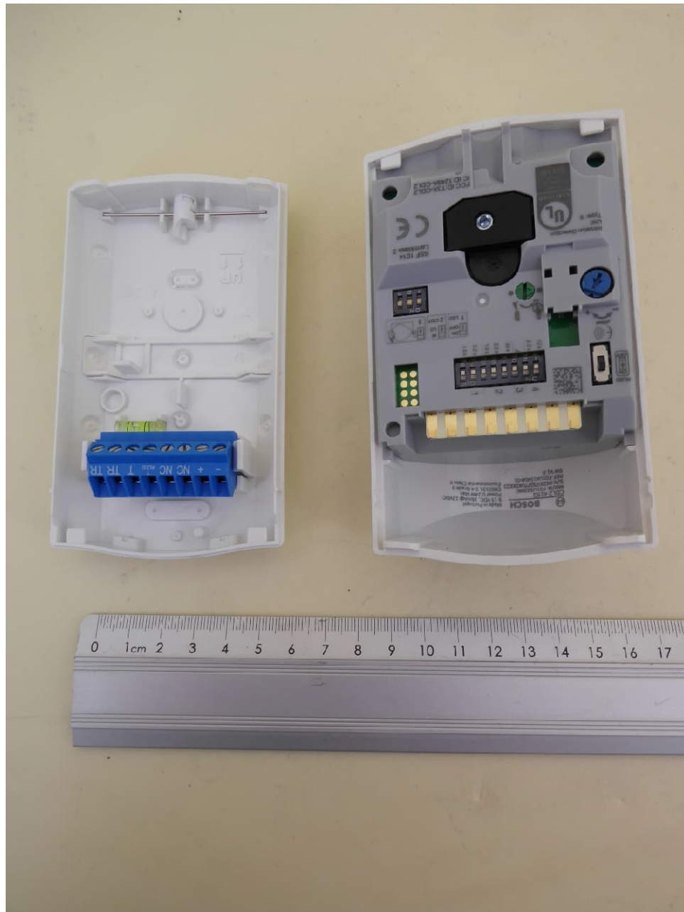
Rear housing panel opened
