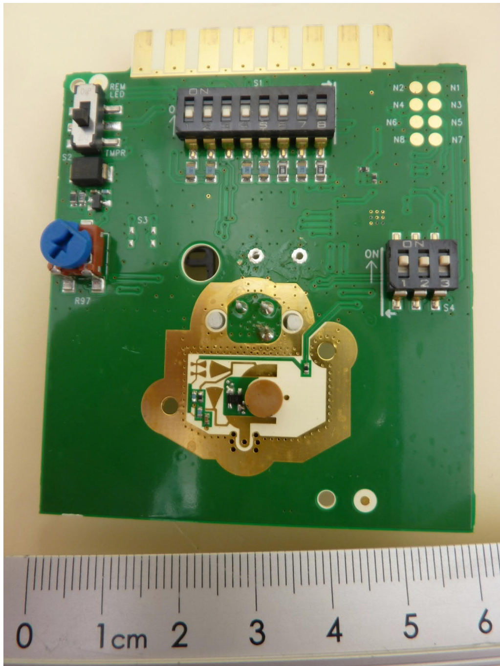
PCB, top view
