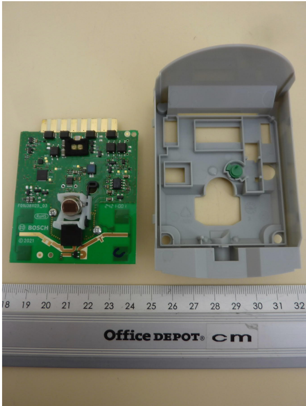
Internal view, PCB removed
