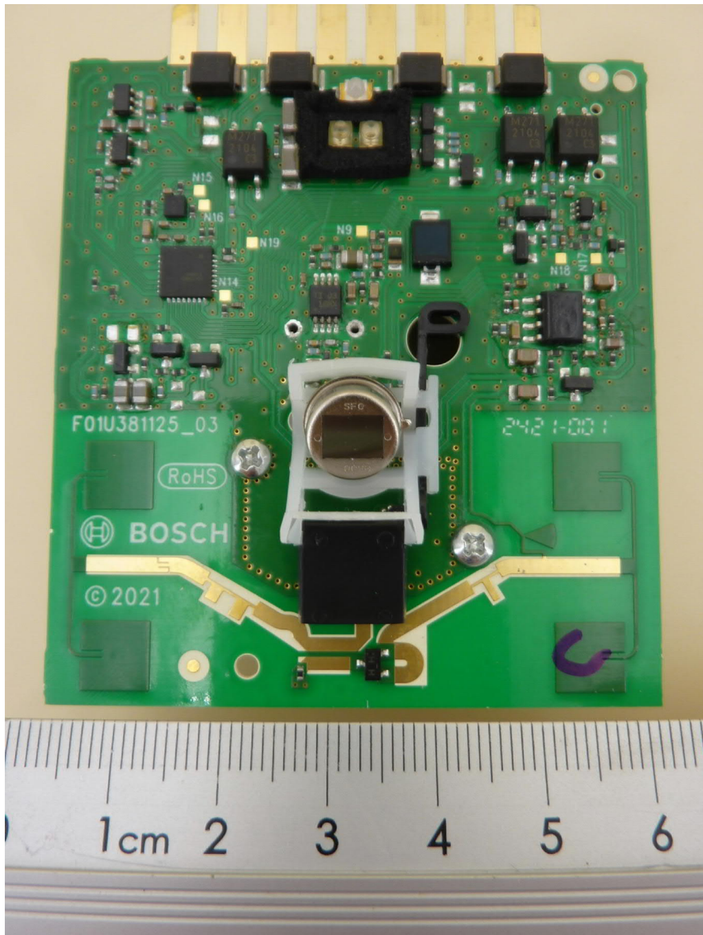
PCB, bottom view
