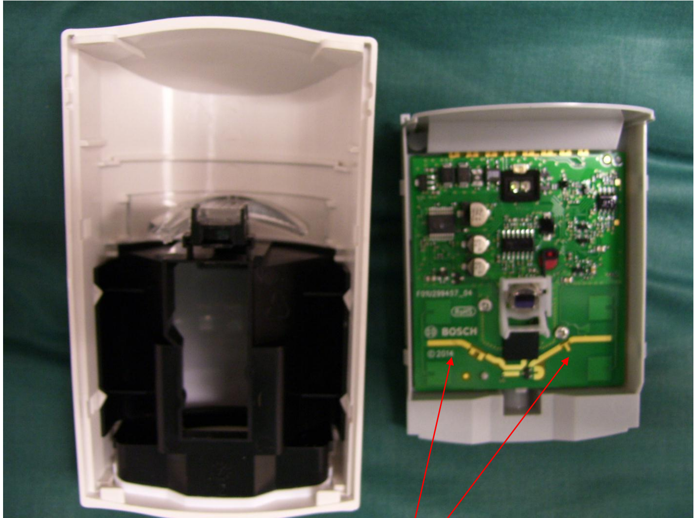
Figure 2: Internal View - Antenna
