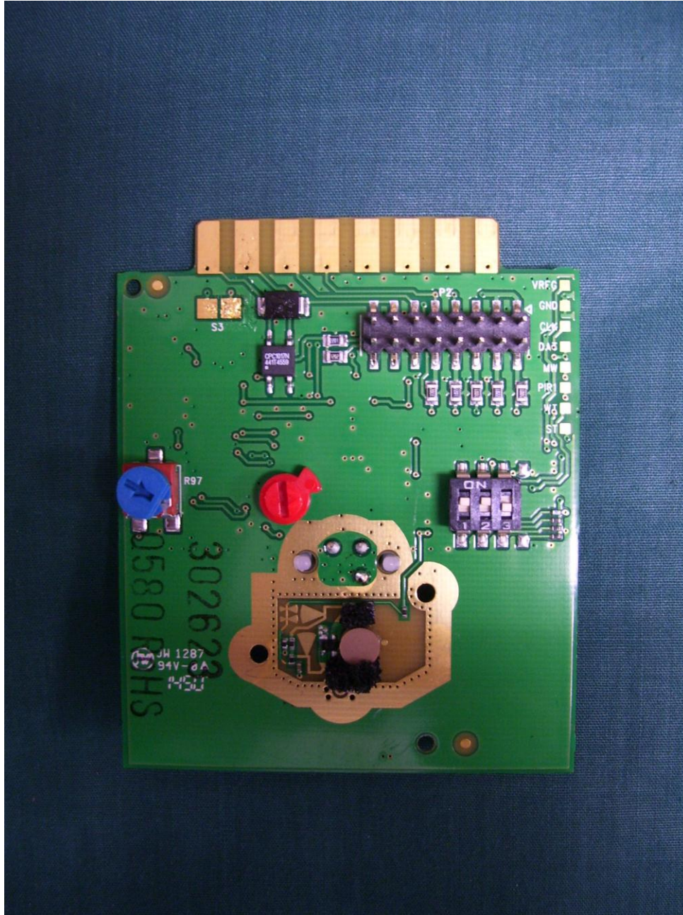
Figure 3: Internal View – Back side of PCB
