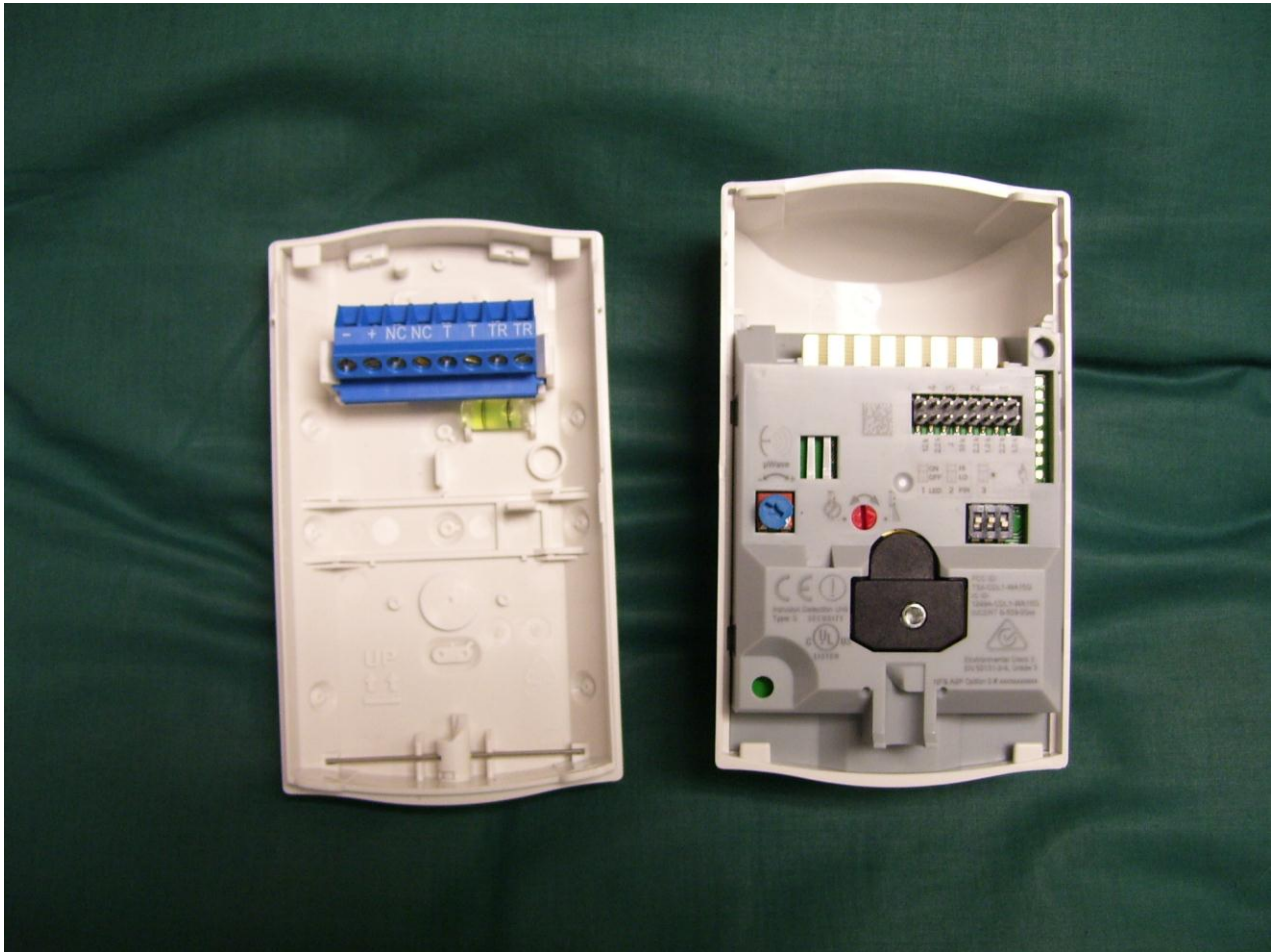
Figure 1: Internal View
