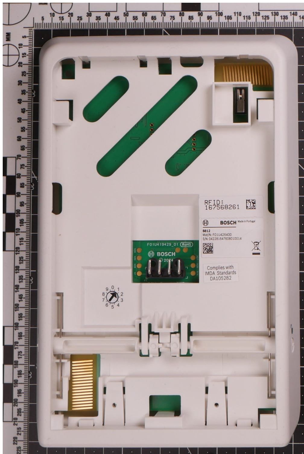
B812 Transceiver Back
