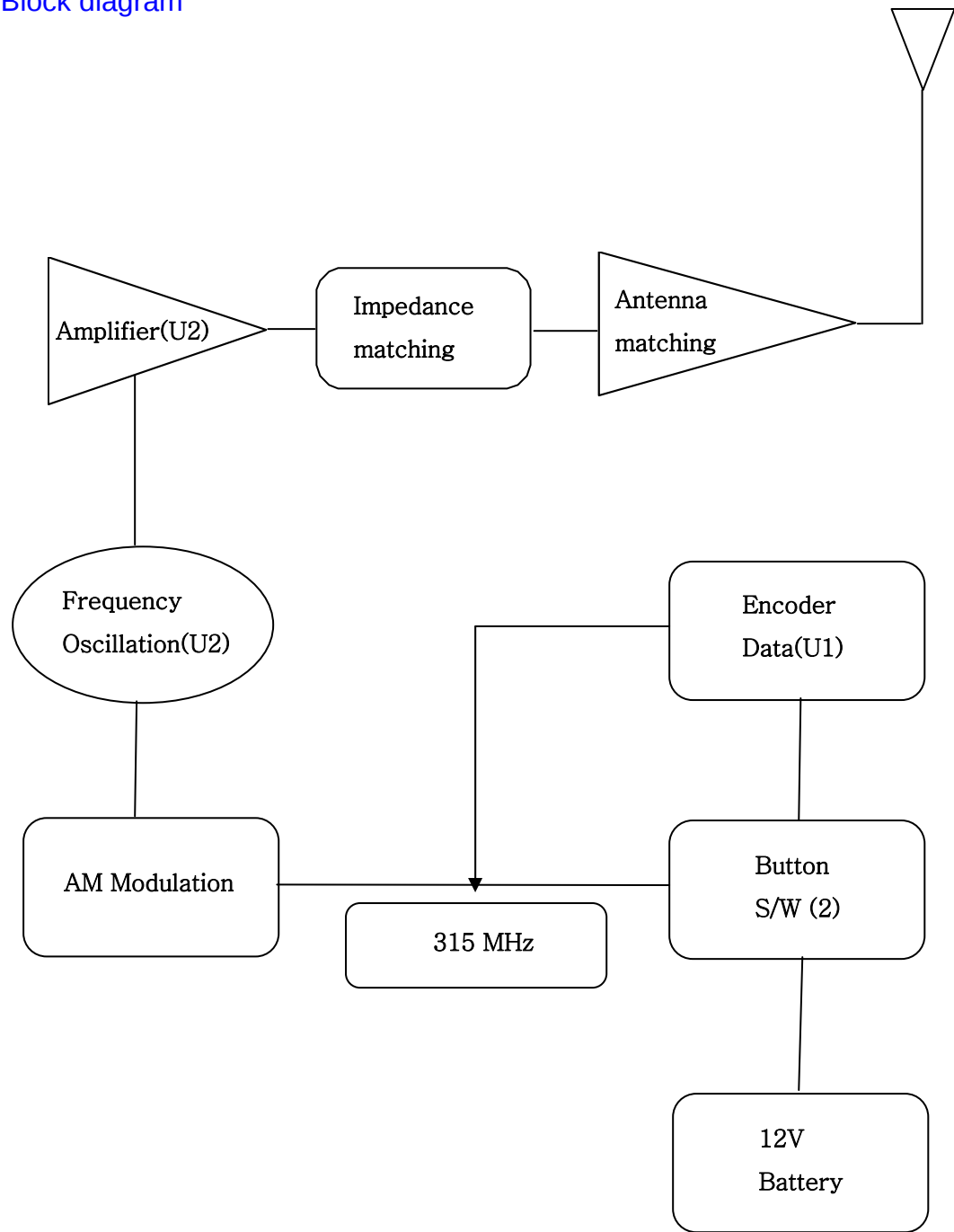
Block diagram
