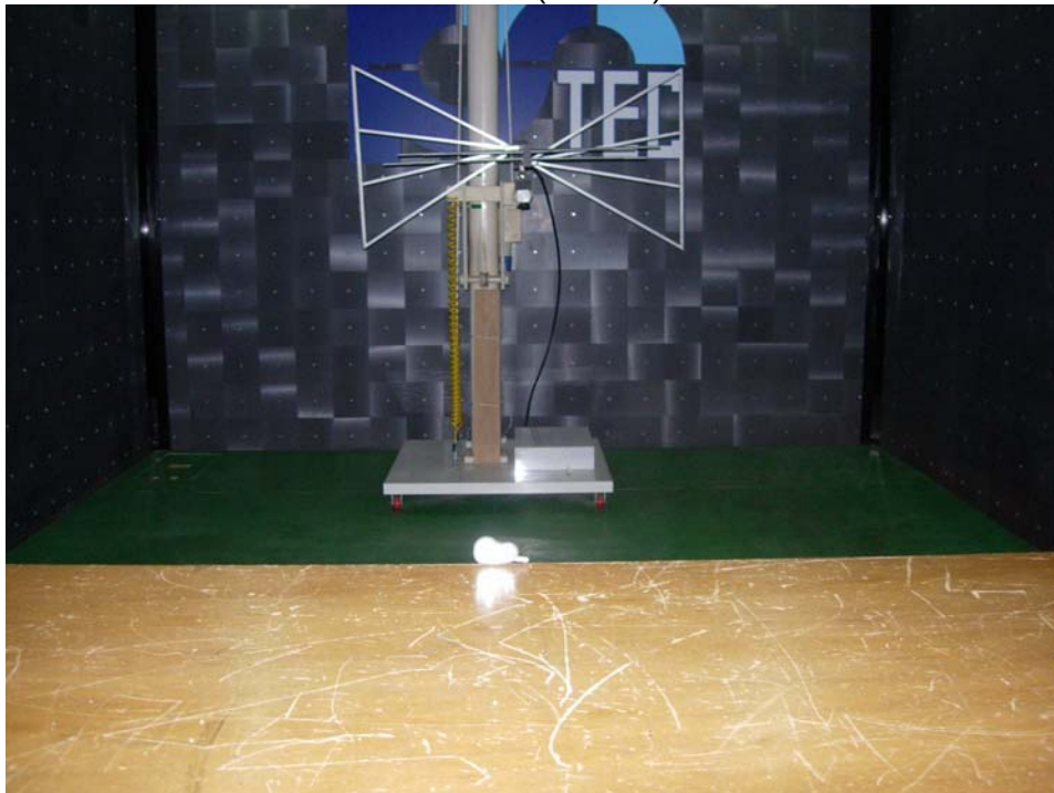
Radiated Emission ( 15.231 ) TX Mode
