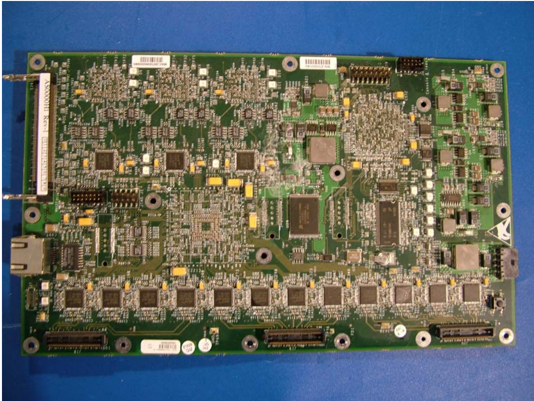
BB board top view
